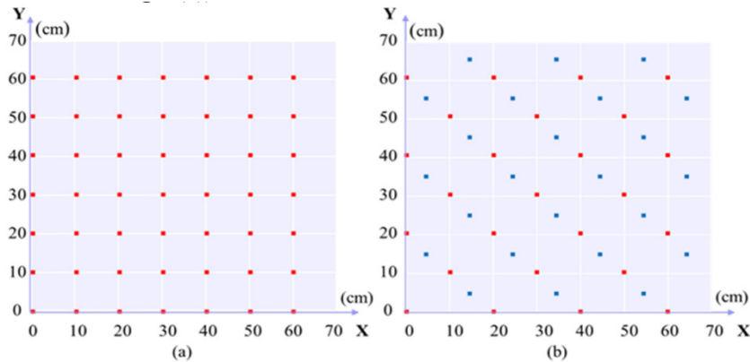
Fig. 4. Sampling points of Detector 1: (a) input for testing different positioning algorithms and (b) training data for the KNN. The 25 red points in (b) coincide with some test points shown in (a).
