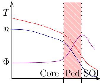
Figure 1.2: An illustration of radial profiles of temperature T , density n and electrostatic potential \Phi in the edge of an H-mode tokamak plasma, with the core, pedestal (“Ped”), and Scrape-Off layer (“SOL”) regions highlighted. See the text for an explanation of the different regions.
