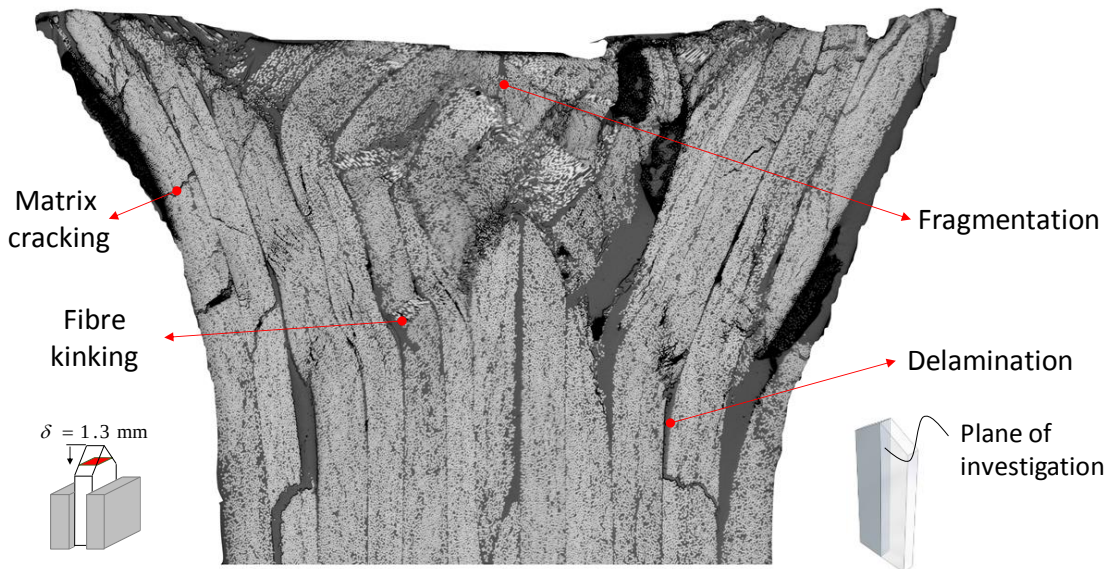
Figure 9. Micrograph of the cross section of a partially crushed flat coupon with fibre lay-up of [\pm 45] showing several crash mechanisms including kink band formation, courtesy of Thomas Bru
