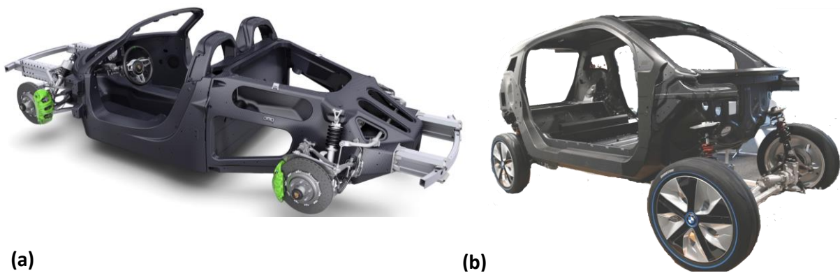
Figure 3. Composite body structure with front and rear steel subframes: (a) Porsche 918 [6]; (b) BMW i3
