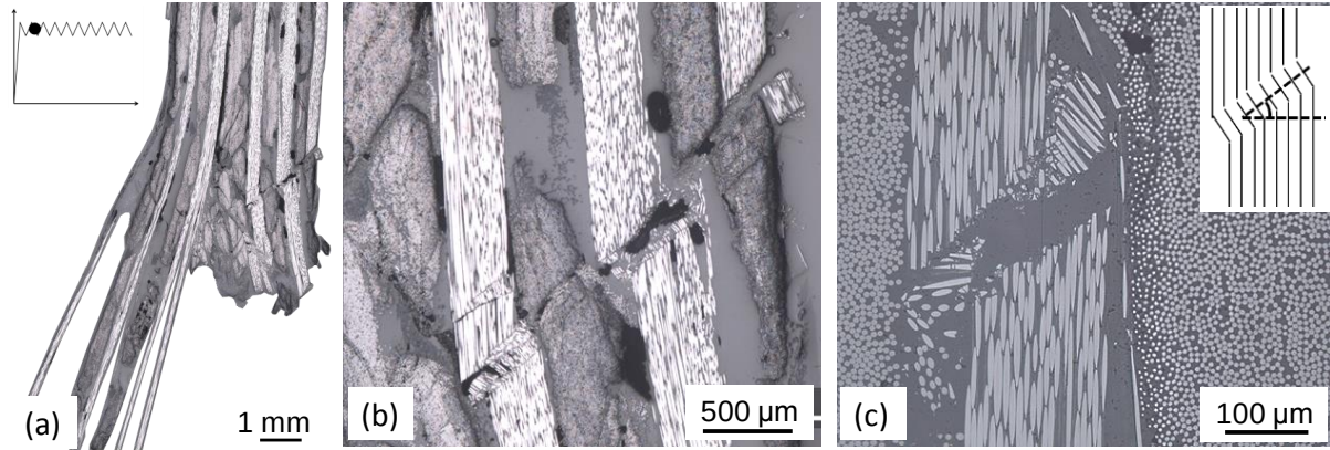
Figure 7. Micrographs through the thickness with different amplifications: (a) Bending failure (left) and compressive failure (right); (b) Kink bands in several bundles with intermediate matrix cracking; (c) Kink bands through a single bundle, adapted from [19]
