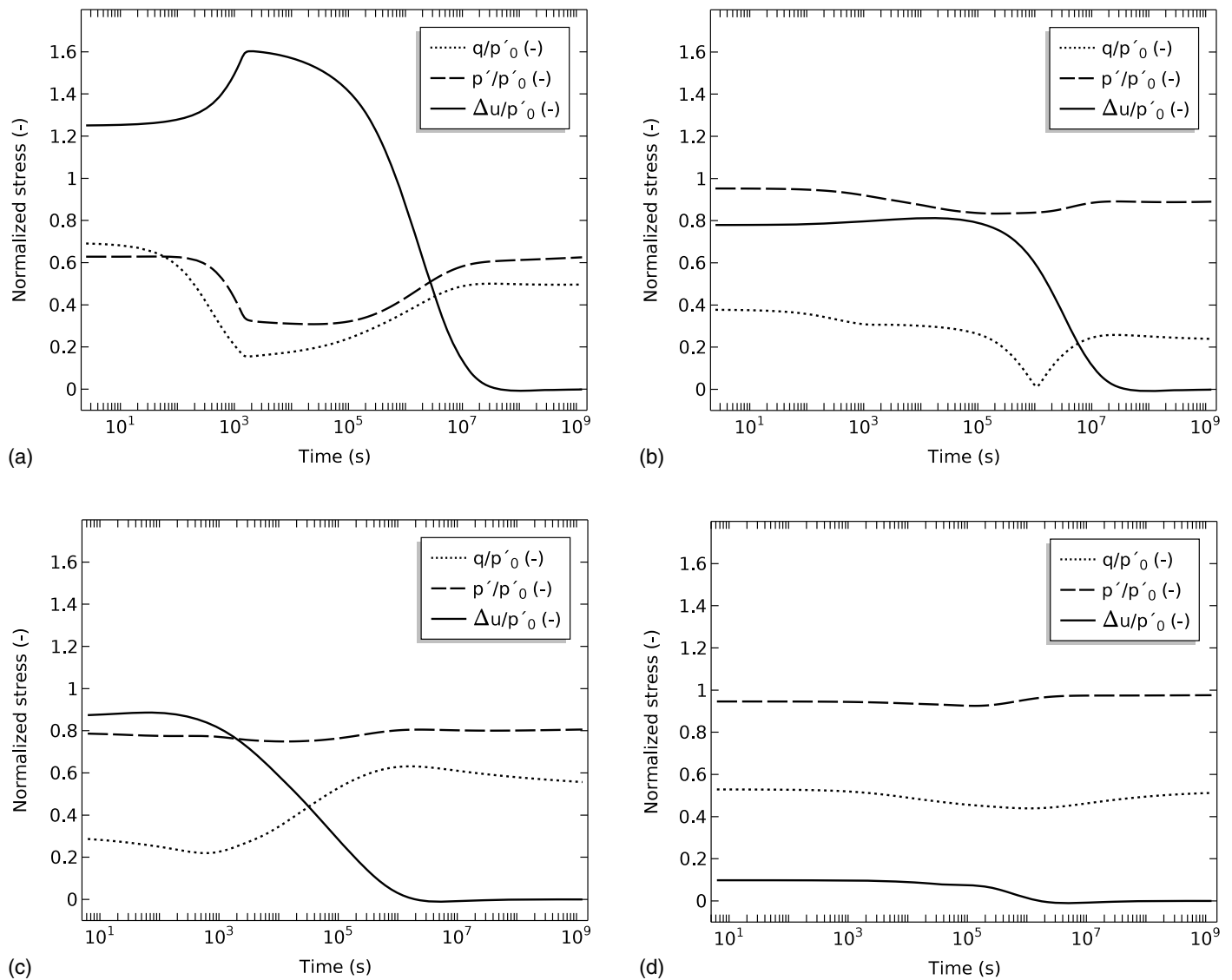
Fig. 2. Normalized mean effective stress p'/p'_0 , deviatoric stress q'/p'_0 , and excess pore pressure \Delta u/p'_0 evolution with time at two different distances from the pile wall, where r = 0 is the center of the pile and p_0 = 35.3 kPa: (a) closed-ended pile, distance = R_{pile} ; (b) closed-ended pile, distance = 3R_{pile} ; (c) open-ended pile, distance = R_{pile} ; and (d) open-ended pile, distance = 3R_{pile} .
