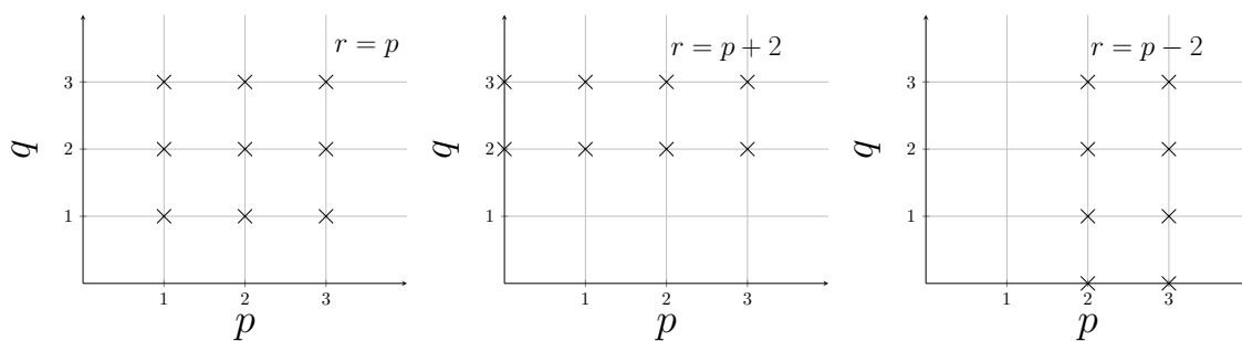
Figure 3. (2,0) towers.
