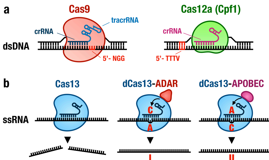
Figure IV-8. Cas12a (Cpf1) and Cas13 features. a. b. Cas13 performs targeted cleavage of an ssRNA substrate. dCas13-ADAR RNA base editing converts A to I (read as G). dCas13-APOBEC RNA base editing converts C to U.
