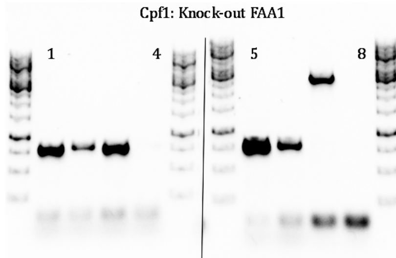
Figure IV-9. Cas12a (Cpf1) proof-of-concept for gene knockout. Colony PCRs for the deletion of FAA1 . Bands shown at 709bp represents correct deletion, while the band at 2900bp for colony 7 shows wild-type genotype.
