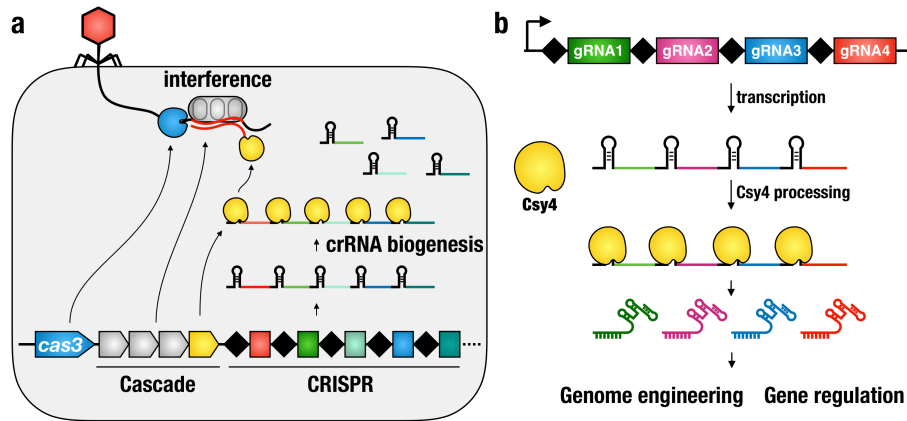
Figure IV-1. Utilization of elements from Type I CRISPR-systems for genome editing and gene regulation. a. Overview of Type I CRISPR-system. The csy complex is usually composed of several csy genes, including csy4 (in yellow). Csy4 processes the CRISPR array to generate several crRNA which will then be used for the interference step against phages. b. Harnessing Type I Csy4 from P. aeruginosa for gRNA multiplexing.
