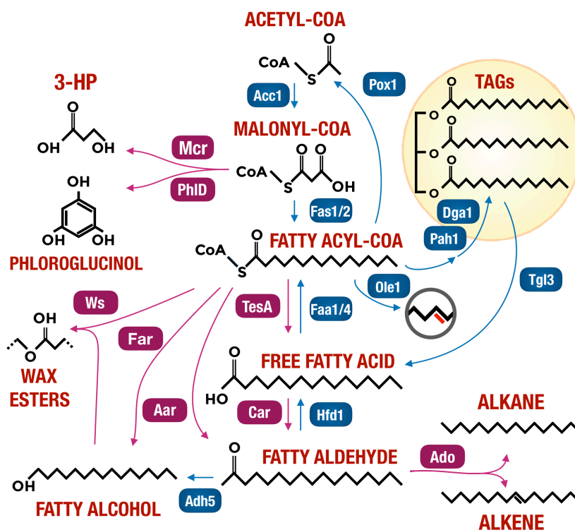
Figure I-8. Strategies for the production of oleochemicals in S. cerevisiae . Acc1: acetyl-CoA carboxylase 1; Fas1/2 : fatty acid synthase 1 and 2; Pox1: fatty-acyl coenzyme A oxidase; Mcr: malonyl-CoA reductase; PhID: type III polyketide synthase; Ole1: fatty acid monodesaturase; TesA: acyl-CoA thioesterase I; Faa1/4: fatty-acid activation 1 and 4; Pah1: phosphatidic acid phosphohydrolase 1; Dga1: diacylglycerol acyltransferase 1; Tgl3: triacylglycerol lipase 3; Ws: wax ester synthase; Far: fatty acyl-CoA reductase; Aar: acyl-ACP reductase; Hfd1: Fatty aldehyde dehydrogenase; Ado: aldehyde-deformylating oxygenase; Adh5: alcohol dehydrogenase 5. Blue arrows: endogenous enzymes from S. cerevisiae , in purple: heterologous enzymes.
