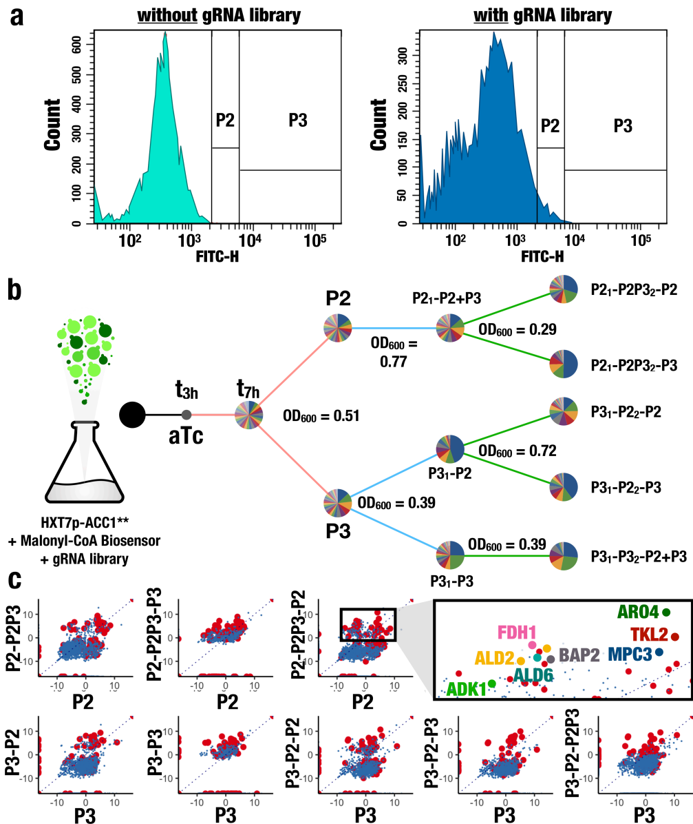
Figure III-7. Three-day sorting strategy of the yeast library. a. After 7 h of culture, the yeast library was subsequently sorted using two different gates, one for medium fluorescence, P2, and one for high fluorescence, P3. The yeast strains without the library (empty plasmid) in the left show few cells on P2 and P3. b. Three-day sorting using the two gates, except for P2 1 -P2+P3 where P2 1 -P2 and P2 1 -P3 were accidentally mixed together. Each pie chart represents the gRNA distribution after the sorting. The colored lines represent the day of sorting: black for day 0; red for day 1; blue for day 2; and green for day 3. c. Log 2 fold-change gRNAs over the initial library (pre-culture). Shown in red are the most enriched gRNAs that were subsequently tested for 3-HP.
