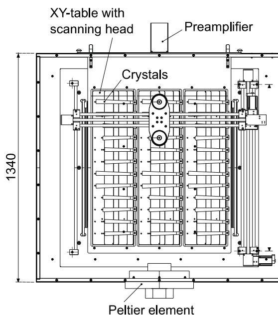
Fig. 2. Top view of the scanning table used for the light output measurements. The setup is enclosed in a thermally insulated and light tight container. A set of 32 crystals can be loaded for consecutive scanning. A typical measurement series uses ten measurement points per crystal and completes, on average, 5 detector modules per hour. The Peltier element mounted on the side port facilitates measurements of the detector response at different temperatures. The size of the setup is indicated by the measure on the left hand side (in mm).
