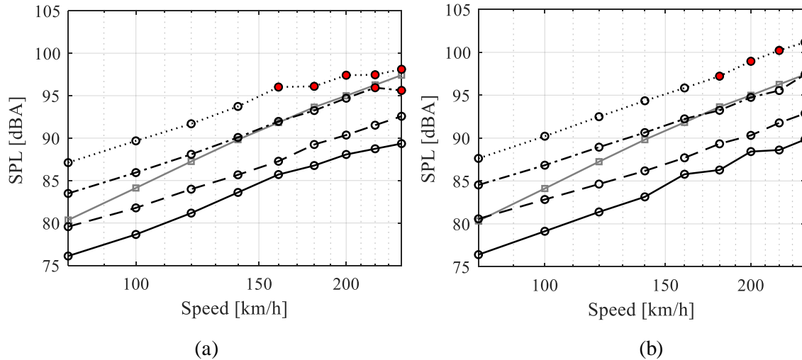
Figure 24. Dip angle 6 mrad ( \text{---}\circ\text{---} ), 12 mrad ( \text{-}\bullet\text{-} ), 18 mrad ( \text{-}\circ\text{-} ), 24 mrad ( \text{\cdots}\circ\text{\cdots} ) and ( \text{---}\square\text{---} ) rolling noise. Rolling noise is calculated for a time window corresponding to 20 m, while the impact noise cases are calculated for a time window corresponding to 0.125 s. Cases with loss of contact are filled in red. (a) facing move, (b) trailing move. The x -axis is given on a logarithmic scale.
