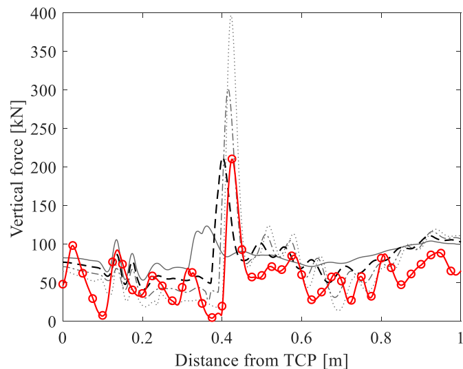
Figure 15. Calculated time history of vertical wheel–rail contact force in the crossing panel. Facing move, axle load 20 tonnes and speed 100 km/h. Results calculated for the pass-by of a S1002 wheel profile on the Loreley crossing (—○—), and on generic crossings with dip angles 6 mrad (—), 12 mrad (---), 18 mrad (-·-·-) and 24 mrad (·····)
