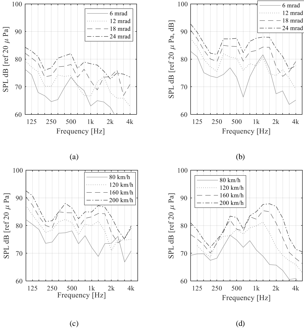
Figure 23. Noise spectra for impact noise and rolling noise simulations at different speeds and dip angles. (a) impact noise at 80 km/h; (b) impact noise at 160 km/h; (c) impact noise at 80 – 200 km/h for 18 mrad dip angle; (d) rolling noise at 80 – 200 km/h
