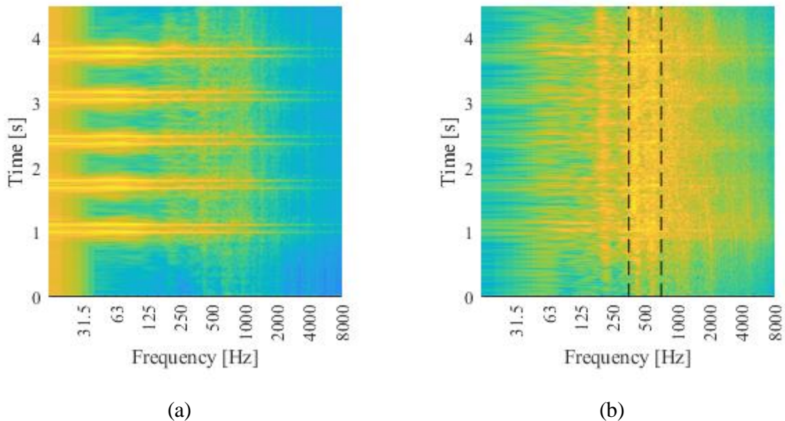
Figure 5. Measured (a) rail vibration level and (b) sound pressure level spectrograms
