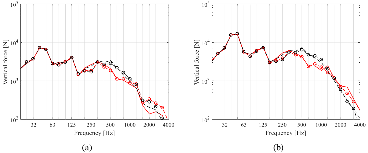
Figure 19. Calculated spectrum of vertical wheel–rail contact force for the pass-by of a wheel with profile S1002 on the generic crossing with dip angle (a) 12 mrad and (b) 24 mrad. Vehicle speed 160 km/h, axle load 20 tonnes and facing move. —: Flexible wheel, facing move; --: Rigid wheel, facing move; -o-: Flexible wheel, trailing move; ···o·: Rigid wheel, trailing move
