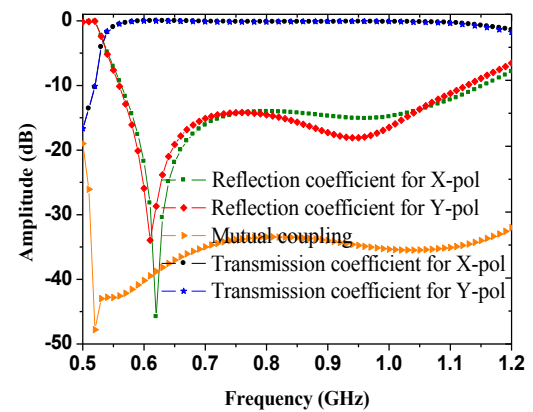
Fig. 2 Simulated data of the bowtie dipole OMT a Transmission coefficient from TEM mode of coaxial port to the first five modes of circular waveguide port b S-parameters of the complete OMT for the dominate mode TE_{11}
