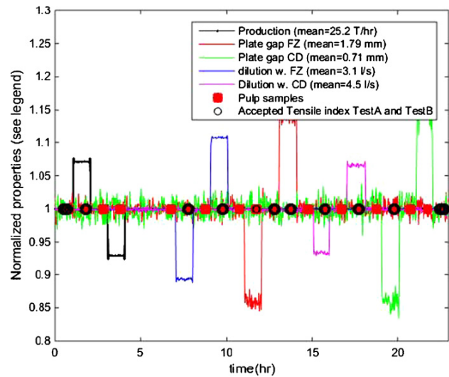
Figure 8: Normalized properties to show where samples for tensile index are taken.
