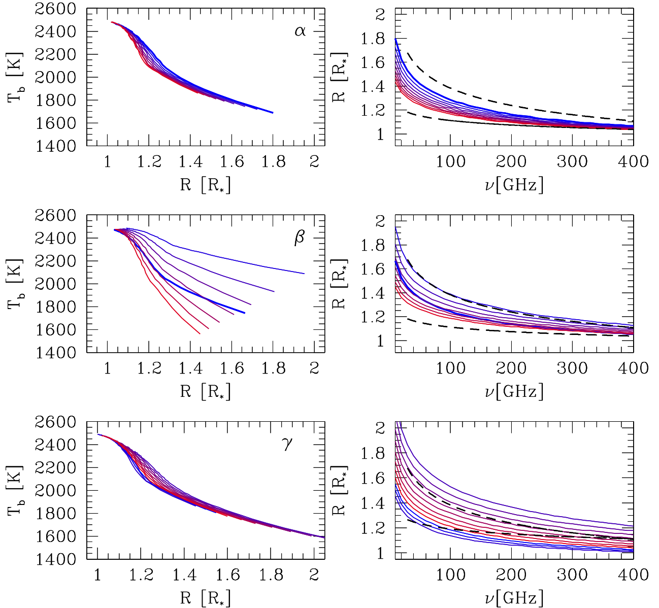
Fig. 9. Brightness temperature vs. size ( left column ) and size vs. frequency ( right column ) relations for model atmospheres (see text) with different power-law slopes for the density profile ( \alpha , top ), temperature profile ( \beta , middle ), and ionisation ( \gamma , bottom ). The two dashed lines indicate the range of the observed slopes of the size vs. frequency relation ( \eta ). Standard parameters are given in Table 3. We vary \alpha from 5 (blue) to 9 (red) in steps of 0.5. We vary \beta from 0.3 (blue) to 1.5 (red) in steps of 0.2 and include the grey atmosphere model (dark blue). We vary \gamma from 2 (blue) to 12 (red) in steps of 1.
