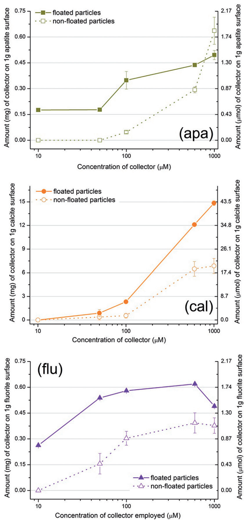
Figure 6. FTIR measurement of \text{C}_{12}\text{MalNa}_2 coated mineral particles (both floated and non-floated).
