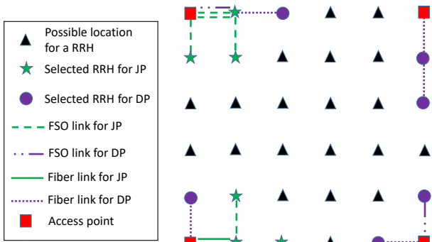
Fig. 6. Example of a JP and DP deployment for capacity requirement 30 [Gbps] and LoS probability 25% with LoS radius 50 [m].
