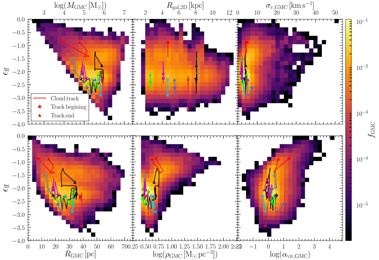
Figure 3. 2D histograms showing how the distribution of \epsilon_{\text{ff}} is correlated with M_{\text{GMC}} , R_{\text{gal,2D}} , \sigma_{\text{v,GMC}} , R_{\text{GMC}} , \rho_{\text{GMC}} and \alpha_{\text{vir,GMC}} of the GMCs identified with the 3D clump finder in the simulation with feedback. All histograms use the same colour scale (shown on the right), which is normalized to the total number of GMCs included in the data. Additionally, each panel shows the evolution tracks of eight randomly selected GMCs.
