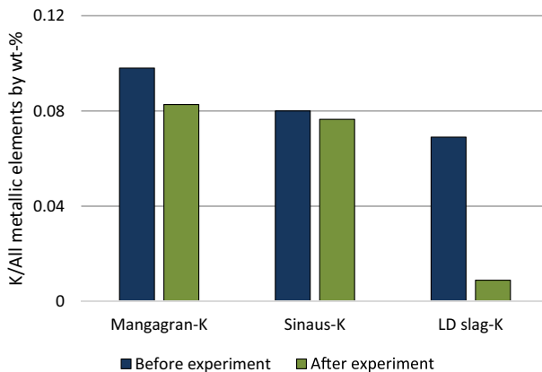
Fig. 13 Weight percentage of potassium in the three impregnated materials before and after the high-temperature experiments
