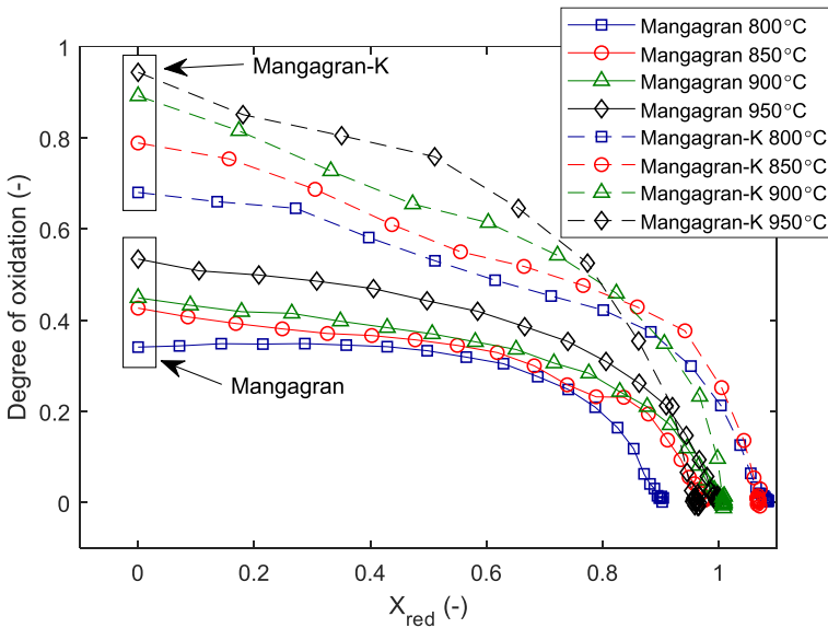
Fig. 5 The degree of gas oxidation as a function of X_{\text{red}} for Mangagran and Mangagran-K at different temperatures
