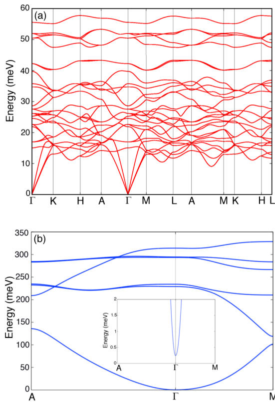
FIG. 4. (a) Phonon band structure of ferromagnetic Fe 2 P. (b) Adiabatic magnon spectra calculated for Fe 2 P using linear spin-wave theory. The inset shows a zoom around the \Gamma point in order to show the spin gap induced mainly by the uniaxial anisotropy.
