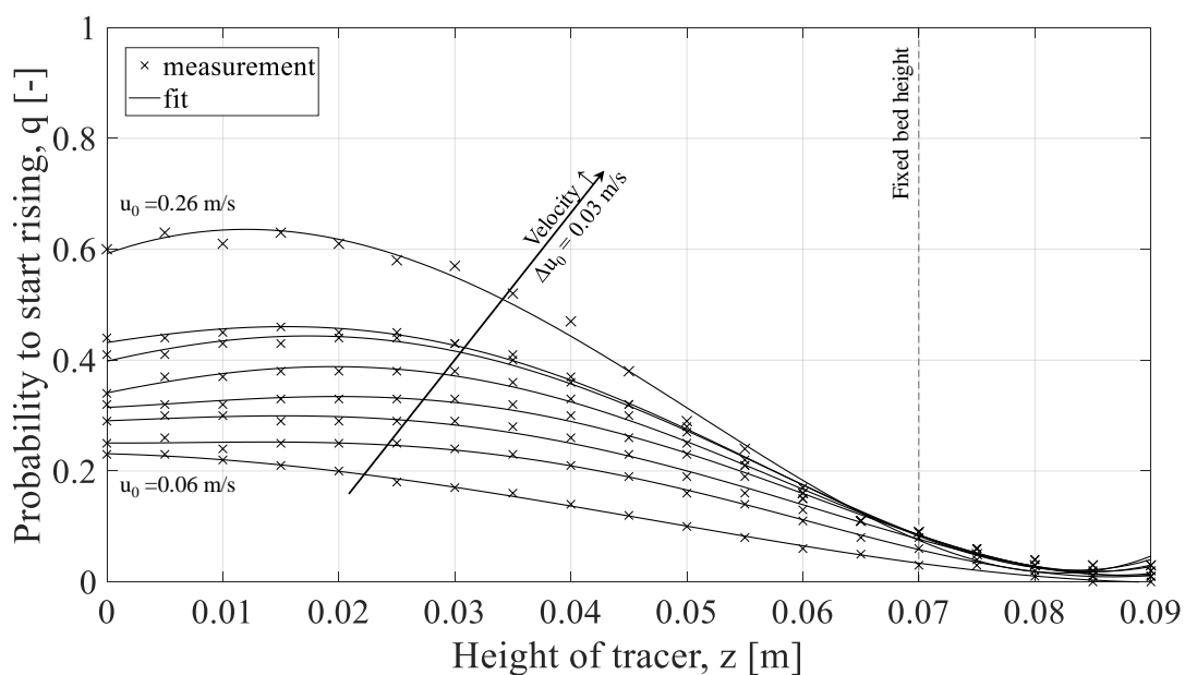
Figure 4.1: Probability of the tracer particle to join the wake region of a bubble, q , over height, z , for different fluidisation velocities (0.06–0.26 m/s). Source: Paper I.
