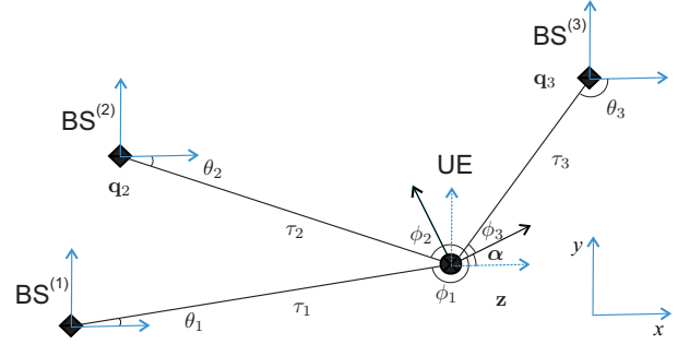
Fig. 1. Communication model showing 3 transmitters (gNB) at location \mathbf{q}_i and receiver (UE) at location \mathbf{z} with LOS delays denoted by \tau_i and angles AoA \phi_i , AoD \theta_i , and the rotation \alpha of the receiver.
