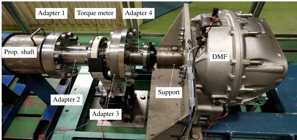
Figure 3: Rig
