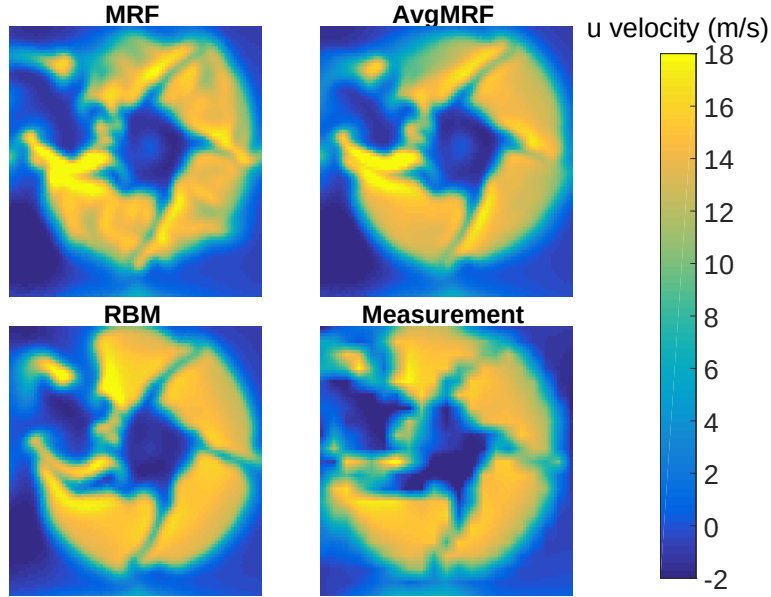
(b) 2800 rpm
