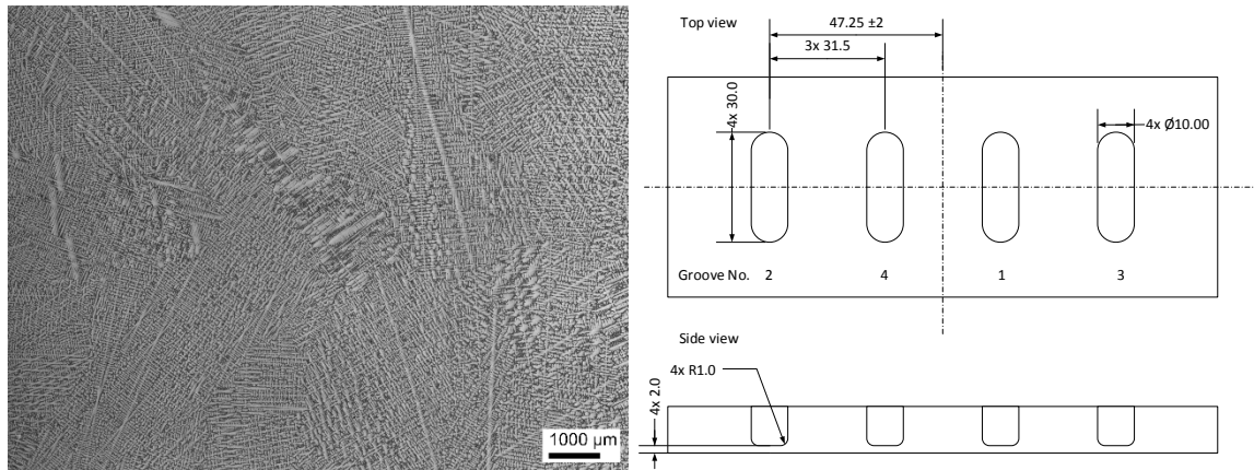
Fig. 1. (a) Microstructure of the cast plate (b) Dimensions and positioning of the welding grooves.
