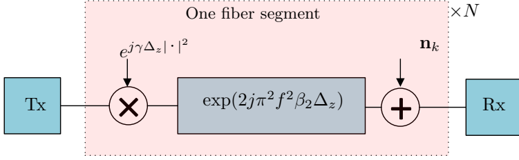
Figure 2.6: Split-step Fourier method for distributed amplification with N segments.
