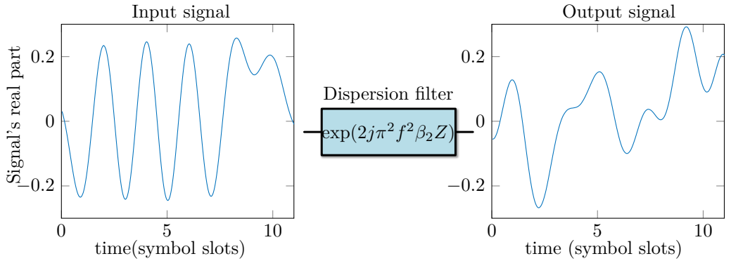
Figure 2.3: Effect of dispersion on a signal after a distance Z > 0 .
