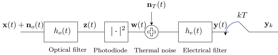
Figure 4.3: A schematic of a noncoherent optical receiver.
