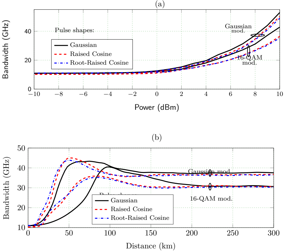
Figure 2.10: Bandwidth (99%) of the propagating signal vs. a) input power and b) distance.
