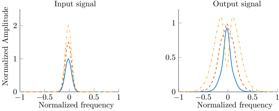
Figure 2.4: Effect of nonlinearity on three pulses with different amplitudes in the frequency domain after propagation.
