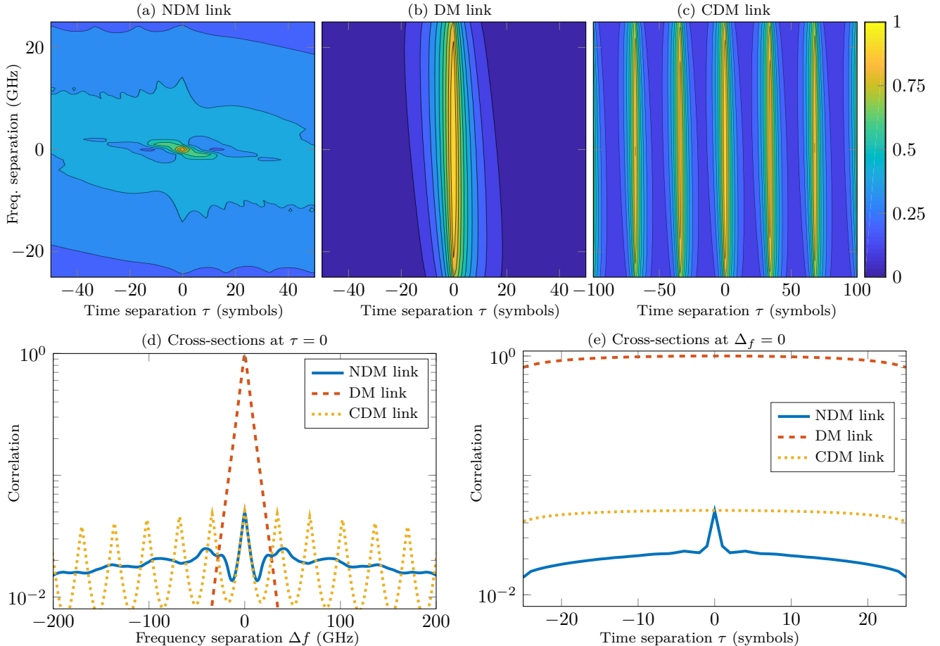
Fig. 2. Correlation function (arbitrary unit) of the XPM phase distortion E[\theta(0, t)\theta^*(\Delta_f, t + \tau)] for NDM, DM, and CDM links with three WDM channels. The cross-sections of the three contour plots at \tau = 0 and \Delta_f = 0 are compared in parts (d) and (e), respectively.
