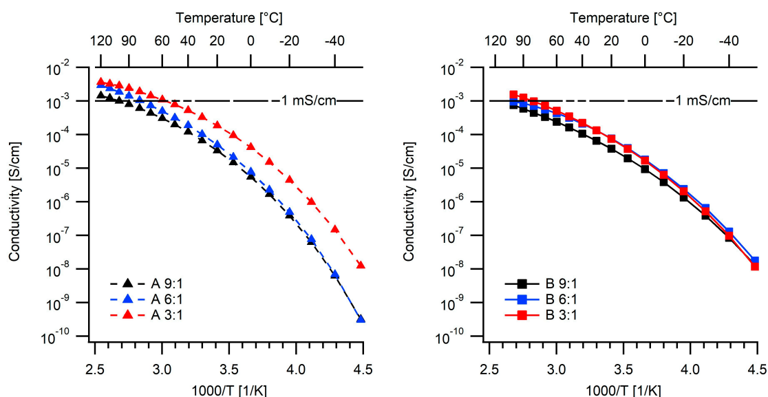
Figure 4. Ionic conductivity cooling traces.
