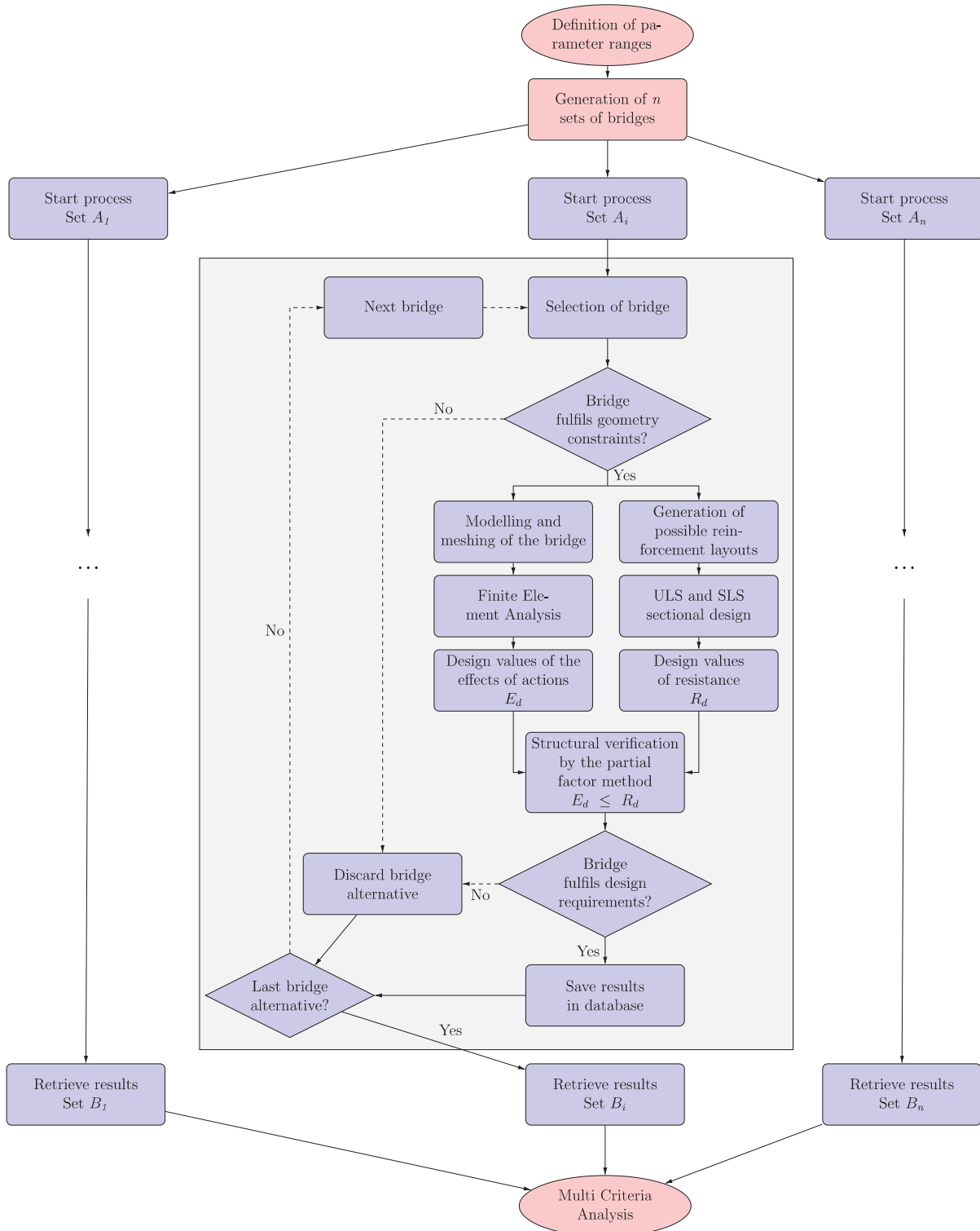
Figure 5.1. Flow chart of python script performing the numerical analyses and controlling the SBPD ( Paper D ).
