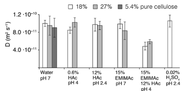
Figure 1: Diffusion coefficients for EMIMAc during coagulation in different coagulation baths for the two solid contents of solution.
