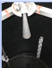
Figure 2. The radar sensor, CS476, operating at 26 GHz.
