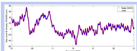
Figure 7. Sea level observations during Dec. 2018.
