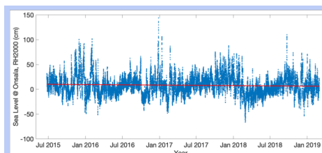
Figure 6. The official time series, based on the radar sensor, is available from the SMHI web page. The sea level at Onsala is mainly determined by the weather. The highest sea level value during this period, approximately +1.5 m, was during the storm Urd in December 2016.
