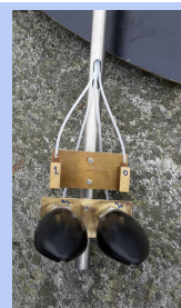
Figure 3. The pneumatic sensors, CS471, have a compressor located in the hut (green unit, left). Each compressor is connected to a nozzle (right) at the bottom of the well via a plastic pipe.
