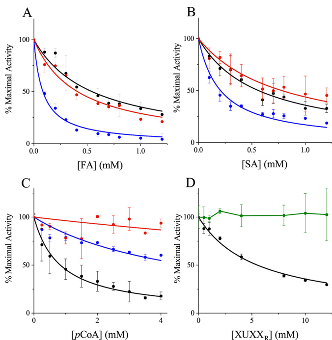
Figure 4. Inhibition of TtCE15A with aromatic compounds and xylooligosaccharides. Inhibition of the WT enzyme activity (black) compared with F174A (blue) and F174D (red) by FA (A), SA (B), and pCoA (C) and inhibition of TtCE15A WT activity (black) compared with W376A (green) by XUXX R (D) are shown. The inhibitors were added in increasing concentrations to 0.4 mM BnzGlcA, up to 1.2 mM FA or SA, 4 mM pCoA , and 12 mM XUXX R . The inhibitory effect of the compounds was calculated by nonlinear regression, fitting Equation 1 (see “Experimental procedures”) to the data (not possible for W376A with XUXX R ). Error bars represent S.D. from the mean value of duplicate measurements. The data are normalized to facilitate comparison, where 100% maximal activity corresponds to the following rates ( v/[E] ): 11.1 (WT), 1.7 (F174A), 0.3 (F174D), and 3.0 s -1 (W376A). Similar or even stronger inhibition by FA and SA was observed for the Phe-174 variants compared with the WT enzyme. However, the variants lacking Phe-174 or Trp-376 were less inhibited by pCoA and XUXX R than the WT enzyme.
