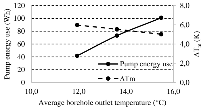
Figure 20. Relation of the borehole water temperature, the \Delta T_m of the panels and the energy use of the pump installed in the building loop for a period of 8 hours and tested under periodic space heat gain conditions
