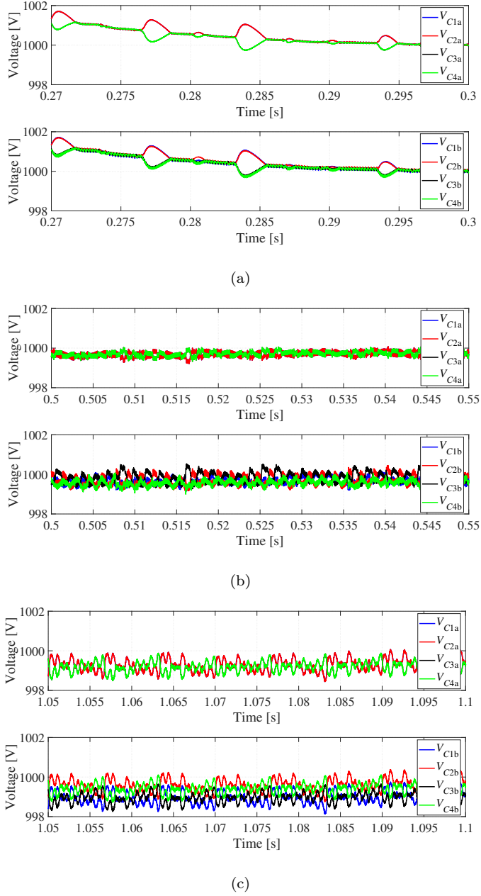
Fig. 4.11: Simulation results of the dc-link voltages when the generator-side 5-level NPC converter operates in (a) region 0, (b) region I and (c) region II of the SVM plane
