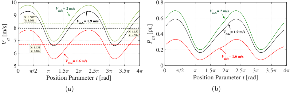
Fig. 2.3: (a) Effective water speed in m/s and (b) turbine power in pu for maximum C_P as a function of the kite's position on the Viviani's curve
