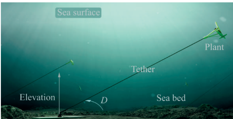
Fig. 1.1: TUSK plant schematic into the sea showing the tether connecting the kite to the sea bed [Property of Minesto AB]
