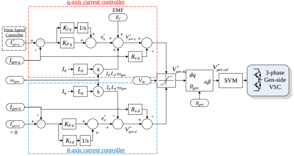
Fig. 2.10: Block diagram of the SG current controller in dq-frame
