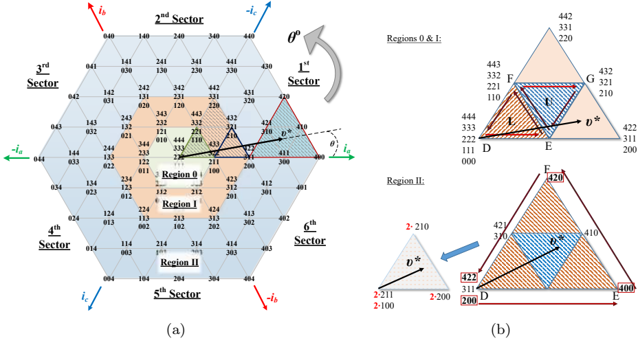
Fig. 4.8: Five-level SVM diagram: (a) space vector plane indicating the regions and sectors; (b) first sector of the SVM plane indicating the switching sequence
