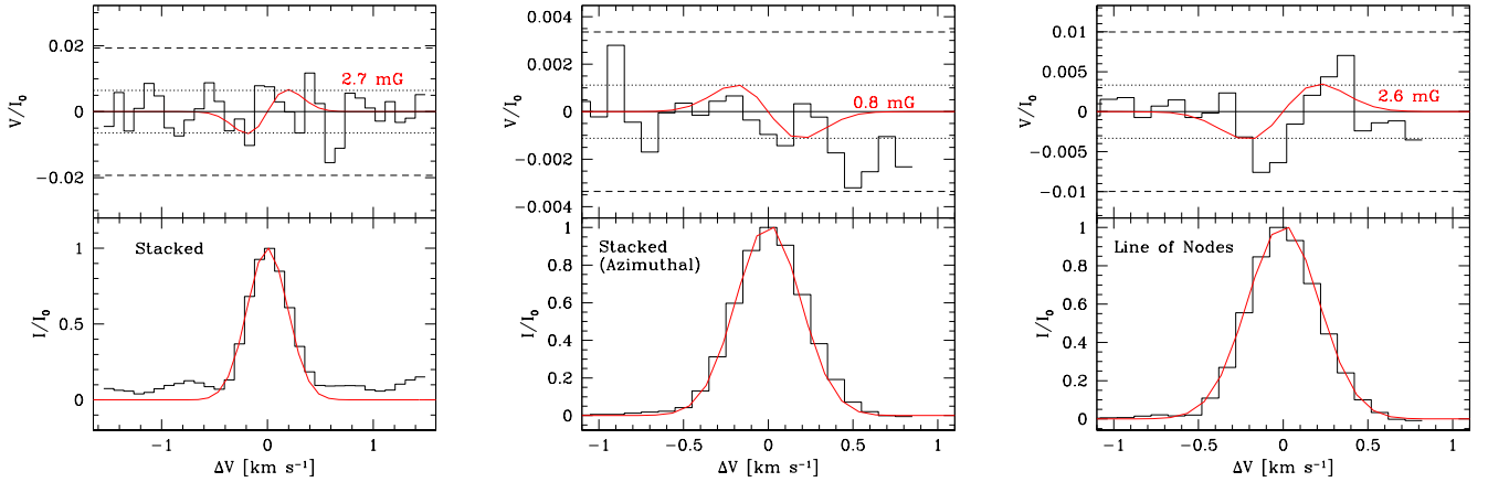
Fig. 2. Total intensity ( I , bottom panel ) and circular polarisation ( V , top panel ) CN spectra. The 1\sigma and 3\sigma limits are indicated by the short and long dashed lines, respectively. Left panel: spectra stacking the nine strongest CN N = 2-1 hyperfine components that we extracted at the position of the strongest emission peak. The 1\sigma limit corresponds to a magnetic field strength |B_z| = 2.7 mG, for which the V -spectrum is indicated in red. The effective line width is 0.45 \text{ km s}^{-1} . The apparent non-zero baseline in the Stokes I spectrum is due to the contribution to the stacked spectrum of hyperfine components that occur within 1.5 \text{ km s}^{-1} of each other. Middle panel: azimuthally averaged spectra obtained by stacking the two strongest CN hyperfine components in our data that are not significantly blended. The rms limit corresponds to a magnetic field strength |B_z| = 0.8 mG, for which the V -spectrum is indicated in red. The effective line width is 0.45 \text{ km s}^{-1} . Beyond +0.5 \text{ km s}^{-1} , the spectrum is affected by a blend with a neighbouring hyperfine component. Right panel: similar to the middle panel, but only for emission along the line of nodes (see text). Here the signature of a toroidal field would be strongest. The fractional rms reached on the V -spectrum is 0.33%. The rms limit corresponds to a magnetic field strength |B| = 2.6 mG, for which the V -spectrum is indicated in red. This corresponds to a toroidal field strength limit of |B_\phi| < 30 mG. The effective line width is 0.5 \text{ km s}^{-1} .
