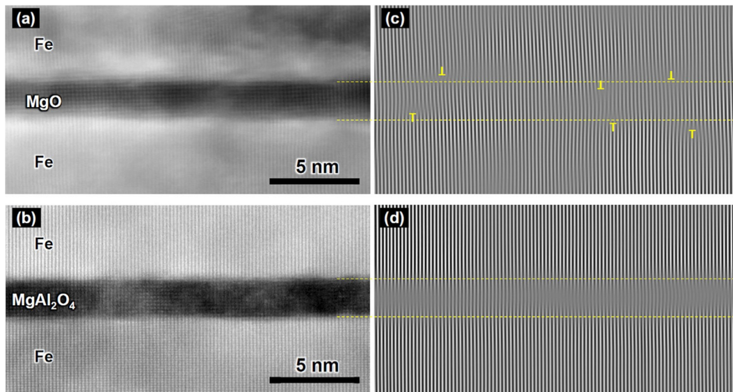
Fig. 36. Cross-sectional ADF-STEM images of epitaxial Fe/barrier/Fe(0 0 1) MTJs: (a) MgO barrier, and (b) MgAl 2 O 4 barrier. (c) [(d)] Outlined images of (a) [(b)] using fast Fourier transform filtering. ⊥ marks indicate edge dislocations.
