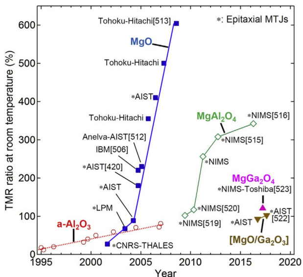
Fig. 34. History of improvement in TMR ratio of oxide barrier based MTJs at room temperature. “a-Al 2 O 3 ” indicates amorphous alumina.
