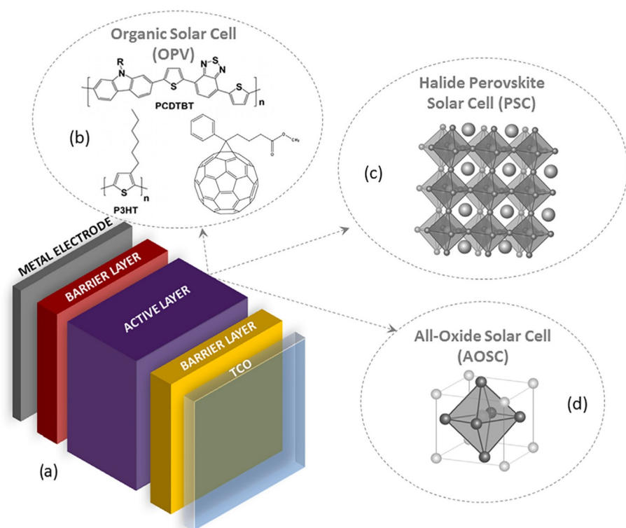
Fig. 41. Oxides in Solar Cells. (a) Schematic representation of a basic solar cell configuration based on five layers: two conducting electrodes labeled as metal electrode and a transparent conducting oxide (TCO), two barrier layers (BL) and the main absorber or active layer (AL). Oxides can be found as barrier layers, as active layer and as electrodes. The name of the solar cell is given by the light absorber material replacing metal electrodes. (b) Organic Solar Cell (OPV), (c) Halide perovskite solar cell (PSC), (d) All-oxide solar cell (AOSC). TCO: Transparent conducting oxides. Modified from [636,637].
