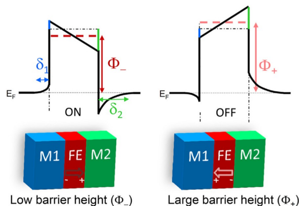
Fig. 23. Tunnel electroresistance induced by the modulation of the potential profile of the ferroelectric (FE) barrier when polarization is reversed in the case of electrodes (M1 and M2) with different effective screening lengths ( \delta_1 and \delta_2 ). The average barrier height is lower, \Phi_- (higher, \Phi_+ ) when the polarization points toward M2 (M1), resulting in the ON (OFF) state resistance. Adapted from [306].
