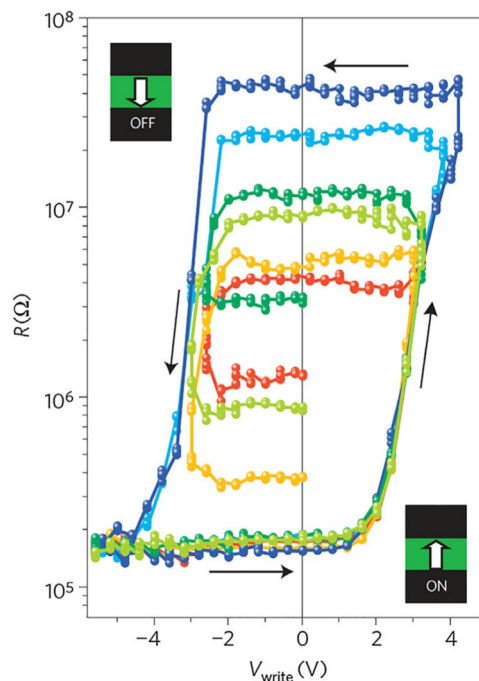
Fig. 3. (La,Sr) \text{MnO}_3/\text{BaTiO}_3/\text{Co-Au} ferroelectric tunnel junction-Dependence of the junction resistance measured at V_{\text{read}} = 100 mV after the application of 20 ns voltage pulses ( V_{\text{write}} ) of different amplitudes. The different curves correspond to different consecutive measurements, with varying maximum (positive or negative) V_{\text{write}} . Taken with permission from [58].
