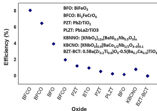
Fig. 45. Examples of photoferroelectric oxides applied in all oxide solar cells. BFCO: Bi 2 FeCrO 6 . BFO: BiFeO 3 ; PZT: PbZrTiO 2 ; PLZT: PbLaZrTiO 3 ; KBNNO: [KNbO 3 ] 12x [BaNi 0.5 Nb 0.5 O 3 ] x ; KBCNO: [KNbO 3 ] 0.9 [BaCo 1/2 Nb 1/2 O 3-δ ] 0.1 ; BZT-BCT: 0.5Ba(Zr 0.2 Ti 0.8 )O 3 -0.5(Ba 0.7 Ca 0.3 )TiO 3 . Details of solar cells with photoferroelectric oxides with PCEs below 1% can be found in [636].
