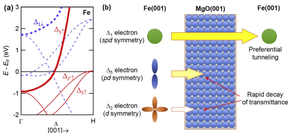
Fig. 35. (a) Band dispersion of bcc Fe in the [001] direction [511]. (b) Schematic illustration of the filtering effect due to the coherent tunneling in an Fe/MgO/Fe(001) MTJ [509].
