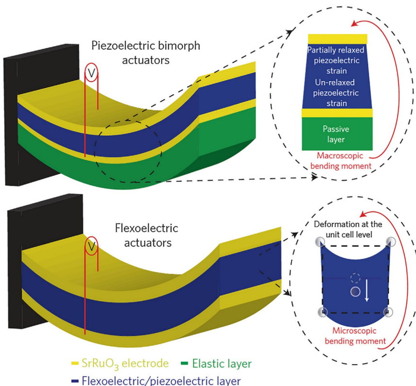
Fig. 5. Schematic comparing flexoelectric actuation and piezoelectric bimorph actuation in nanoscale actuators. In a piezoelectric bimorph actuator, a homogeneous mechanical strain is generated on application of an electrical voltage to the piezoelectric layer. The mechanical clamping induced by the non-piezoelectric layer creates a strain gradient across the structure, converting the piezoelectric strain into a flexural motion. On the other hand, any dielectric sandwiched between the electrodes can, in principle, act as a flexoelectric actuator. In this case, the bending moment arises from a symmetry-breaking strain gradient generated at the unit cell level. Taken with permission from [62].
