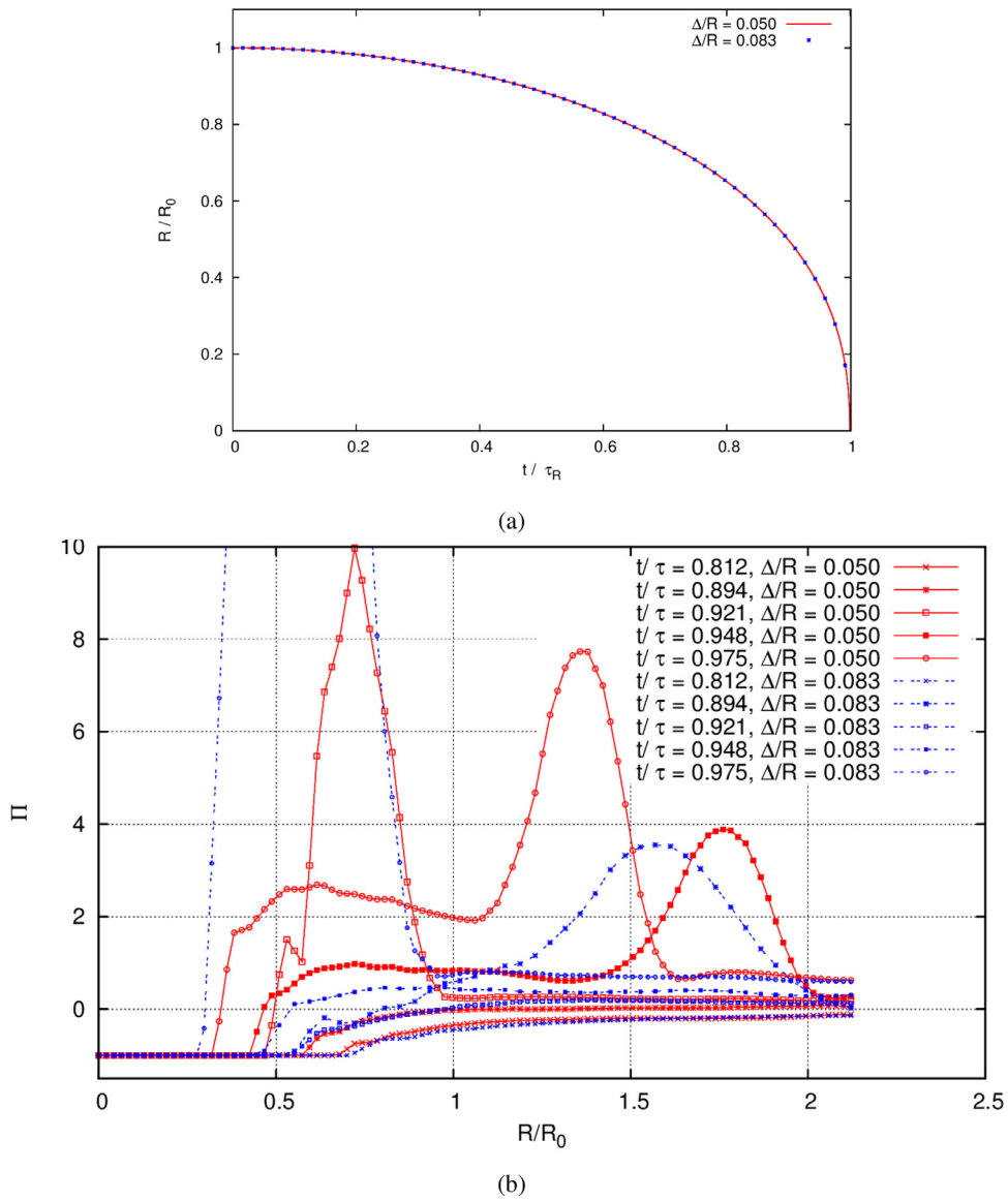
Fig. 6. Domain discretization effect on the equilibrium model; (a) bubble radius; (b) pressure profile.
