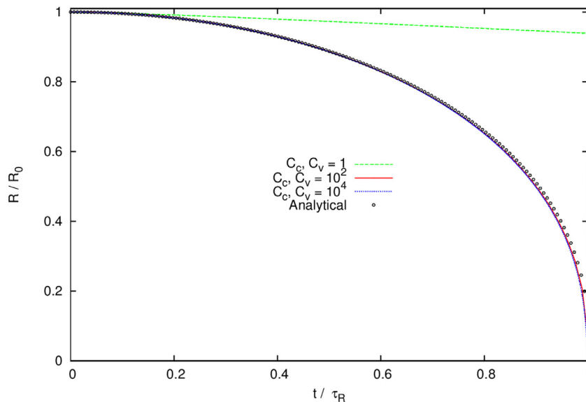
Fig. 7. Validation of the finite mass transfer model with different coefficients in predicting the evolution of the bubble radius.
