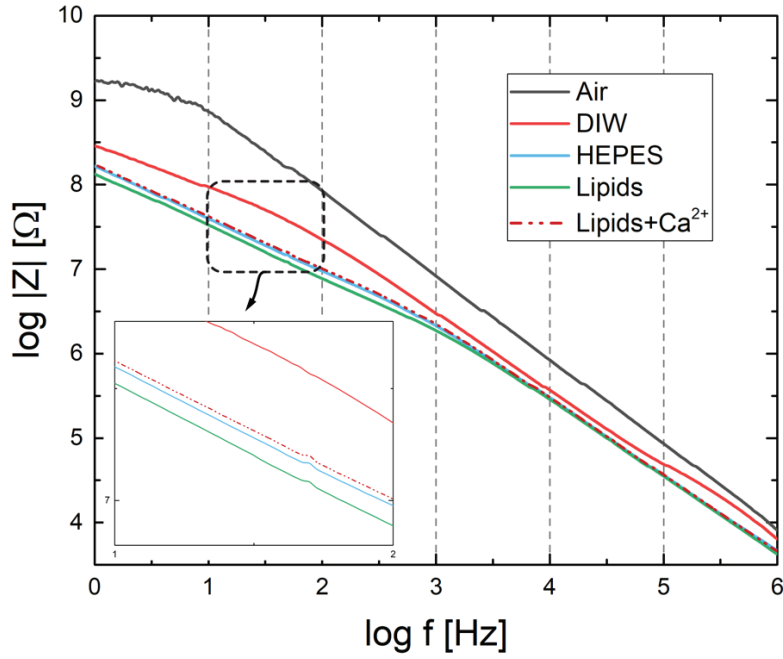
Figure 50. Bode plot of impedance spectra for different analytes. An inset in the bottom left corner is a zoomed-in region of 10 Hz – 100 Hz response from the same plot.
