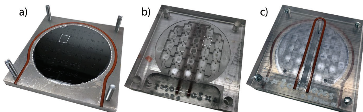
Figure 56. Photographs of the mold used for fabrication of the microfluidic system. a) Bottom part of the mold. Contour of the 4" master wafer is outlined with the white circle, while contour of the individual SAR chip is outlined with the white square; b) top part of the mold with white square outlining the PDMS microfluidic system; c) assembled mold.
