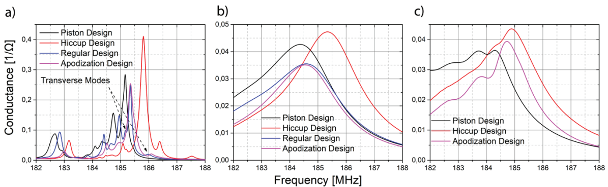
Figure 29. Close-in resonance conductance of the SAW resonators a) in air; b) bonded with 1 cm thick PDMS
