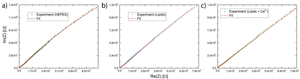
Figure 51. Nyquist plot of EIS response for data obtained experimentally vs. their fit for a) HEPES; b) SLB and b) SLB+Ca 2+ .
