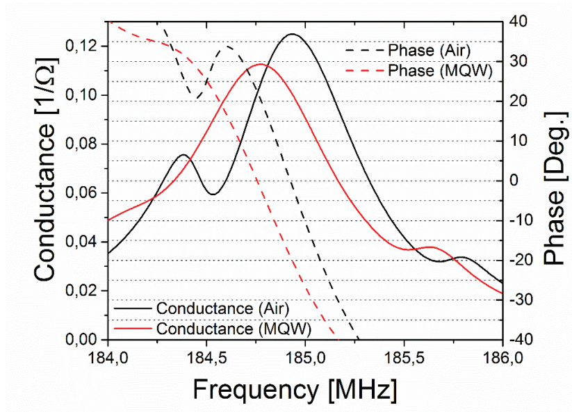
Figure 31. Close-in resonance conductance of the fabricated SAR sensors. The black curve represents the measurement in air-filled, and the red curve in water-filled microfluidic containers. MQW refers to Milli-Q-purified water [126].
