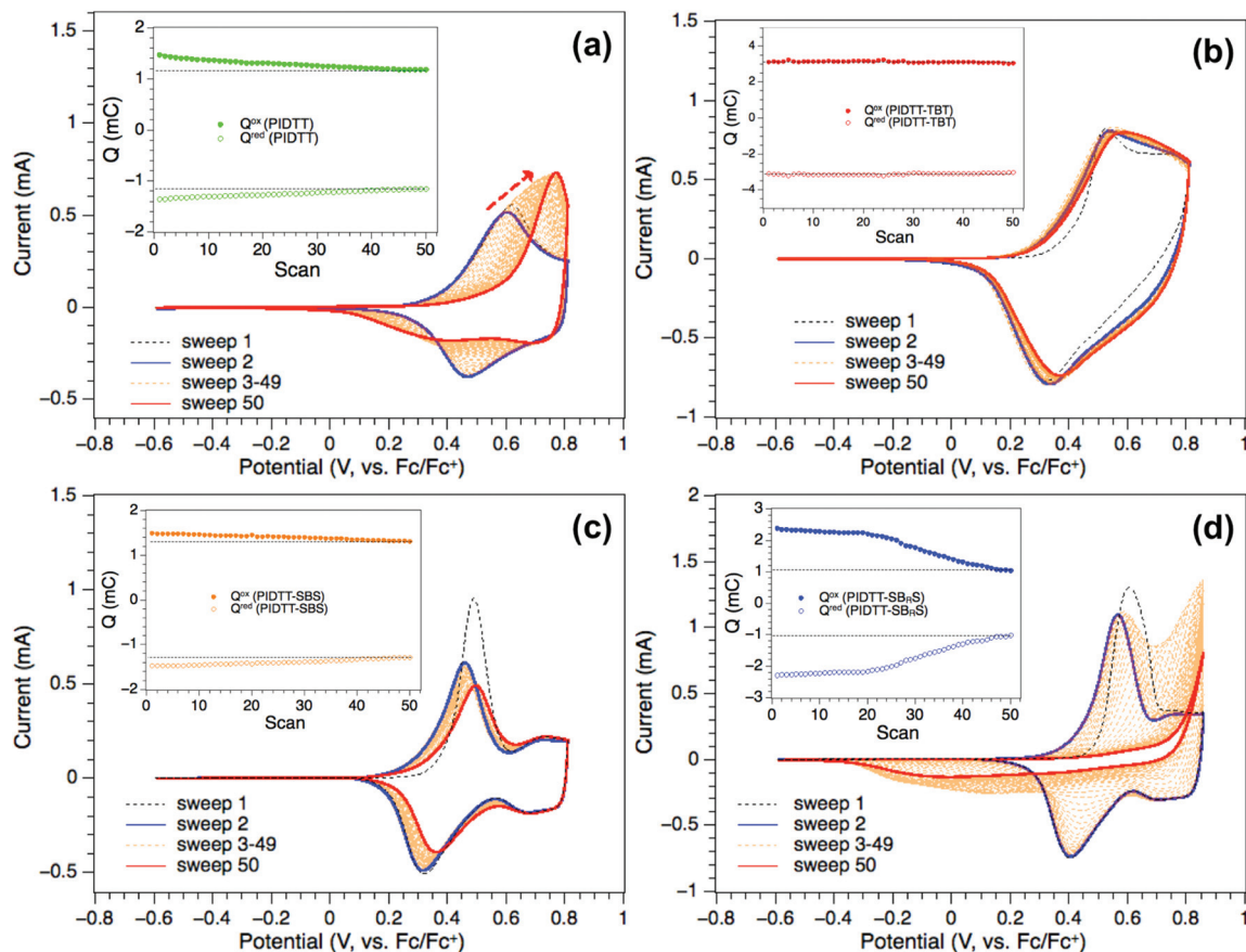
Fig. 4 50 consecutive cyclic voltammetry sweeps of the anodic oxidation of (a) PIDTT, (b) PIDTT-TBT, (c) PIDTT-SBS and (d) PIDTT-SBR S films at a scan rate of 100 mV s -1 . All films exhibit the typical “memory effect” of conducting polymers (first scan effect, sweep 1 in a–d, see also Fig. S11, ESI†). 46 The calculated anodic charges during the forward (solid symbols) and reverse scans (empty symbols) at the respective scan number are shown in the insets.
