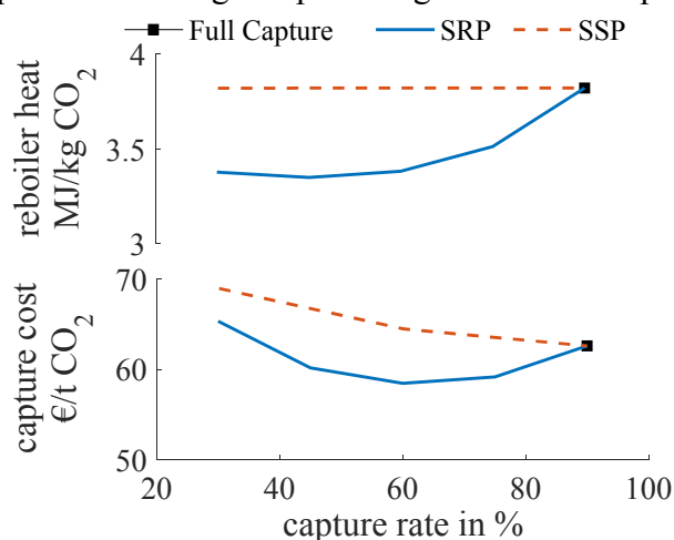
Figure 4-3: Comparison of design paths for partial capture, showing the reboiler heat demand (top) and specific capture cost (bottom) for the separation rate path (SRP) and split stream path (SSP), as compared to a 90% full capture design. The CO 2 concentration in the absorber feed is 20 vol.%. Note that the ordinates do not start from zero. Source: Paper I.
