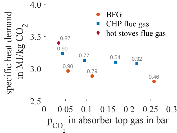
Figure 5-1: Specific heat demand for 30 wt.% MEA absorption from a blast furnace gas (BFG), the flue gas from a combined heat and power (CHP) plant, and the flue gas from the hot stoves with dependence upon the partial pressure of \text{CO}_2 in the lean gas exiting the absorber. The data labels indicate the separation rates of \text{CO}_2 in the absorber (in %).
