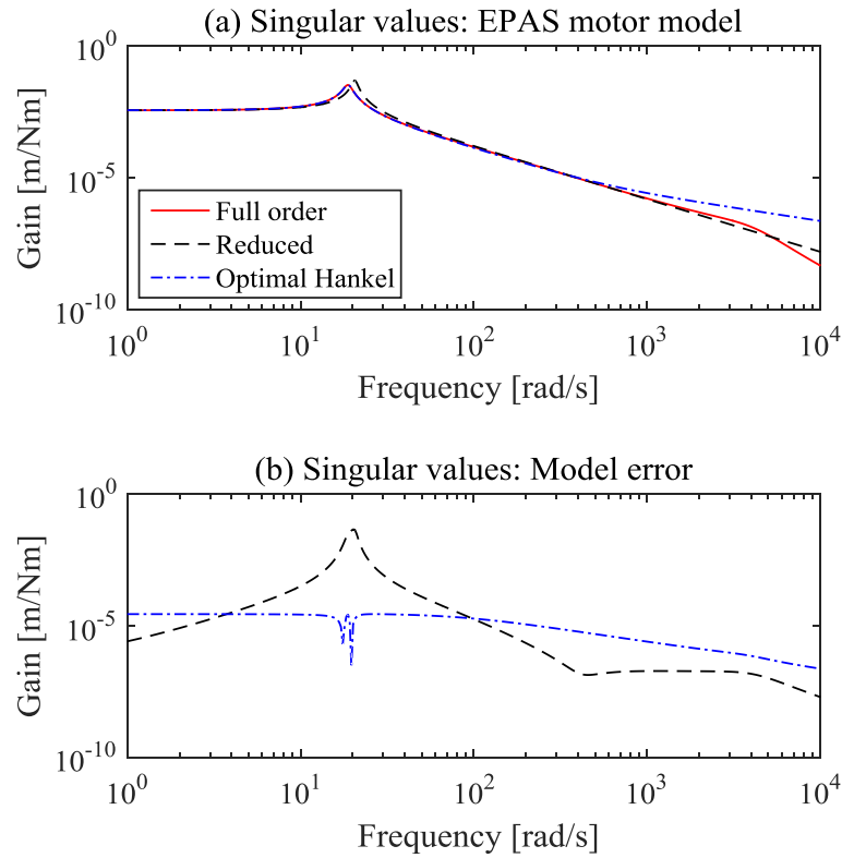
Figure 2.4: (a) Singular values (frequency plot) of full order, reduced order and optimal Hankel EPAS motor model. (b) Singular values of the error system ( \mathbf{G}(s) - \mathbf{G}_a(s) ) for approximated models; reduced lower order and optimal Hankel.
