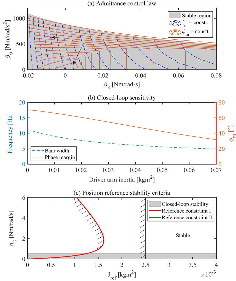
Figure 3.13: SbW-FFb admittance control design results. (a) Stability constraint between the feedback control gains \beta_0 - \beta_3 from Eq. (3.11). The ‘blue’ colored --- lines represent constant bandwidth ( f_{in} ) and the ‘orange’ colored — lines represent constant phase margin ( \phi_m ). The arrows indicate the direction of increasing f_{in} and \phi_m . (b) Closed-loop sensitivity of driver arm inertia on f_{in} and \phi_m . (c) The ‘Reference constraint I’ is stability criteria in Eq. (3.14) between admittance reference inertia and feedback gain \beta_2 . The ‘Reference constraint II’ represents J_{ref} \geq J_{mot} \forall \beta_2 \geq 0 . The unstable regions are hatched for convenience. The ‘Closed-loop stability’ criteria is derived using Eq. (3.11)
