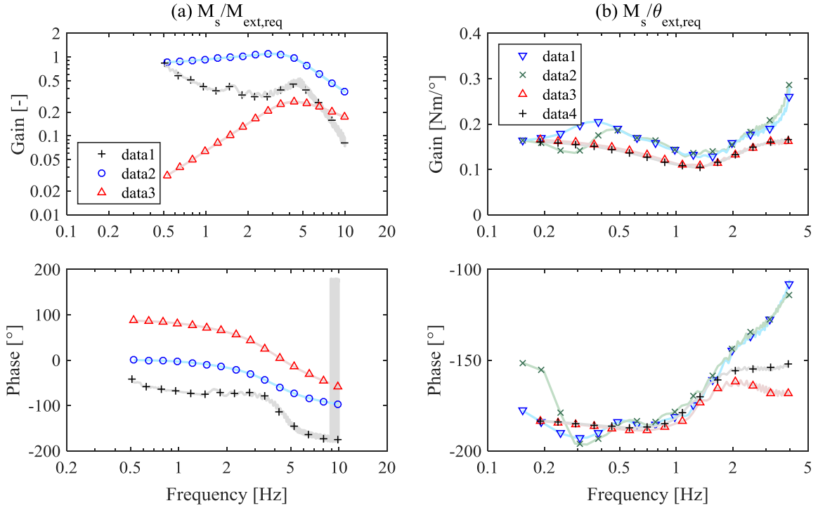
Figure 4.2: (a) Motor torque overlay: Frequency response of M_s/M_{ext,req} for test Case III(a) at 75 km/h vehicle speed. The plot details are: data1 – EPAS open loop, data2 – SbW-FFb open loop and data3 – a typical closed-loop control. (b) Angular position overlay: Frequency response of M_s/\theta_{ext,req} for test Case III(a) at 75 km/h vehicle speed. The plot details are: data1 – EPAS impedance control, data2 – EPAS admittance control, data3 – SbW-FFb impedance control and data4 – SbW-FFb admittance control.
