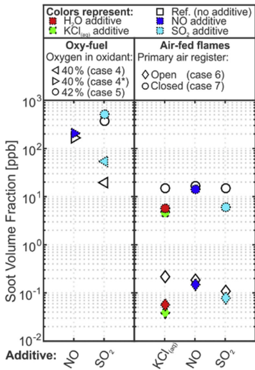
Fig. 5. The effects of different additives ( \text{KCl}_{(\text{aq})} , \text{H}_2\text{O} , \text{NO} , and \text{SO}_2 ) to some of the investigated oxy-fuel and air flame cases. The results have been averaged from calibrated LII images. Case 4* has the same settings as the normal case 4, however, with significant increased soot concentrations probably due to a thermal effect after running the furnace for a full day.
