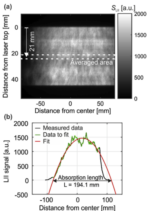
Fig. 2. (a) presents the first step of the calibration procedure, i.e. calculation of the average LII signal used in step 2 and for attaining the corresponding LII signal to the measured soot volume fraction. (b) shows the second step of the calibration procedure, where an estimation of the absorption length based on averaged LII signals are performed.
