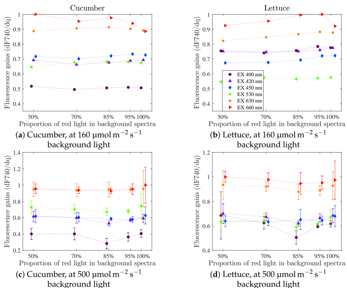
Figure 6. Fluorescence gains for each of the six LED colours when background light quality varies from 50 to 100% red light. The upper row is data from set A, and the lower row is for parts of set B. Left column is measurements on cucumber and right column is on lettuce. The bars in the lower plots represent \pm one standard deviation calculated from the measurements at the current light setting.
