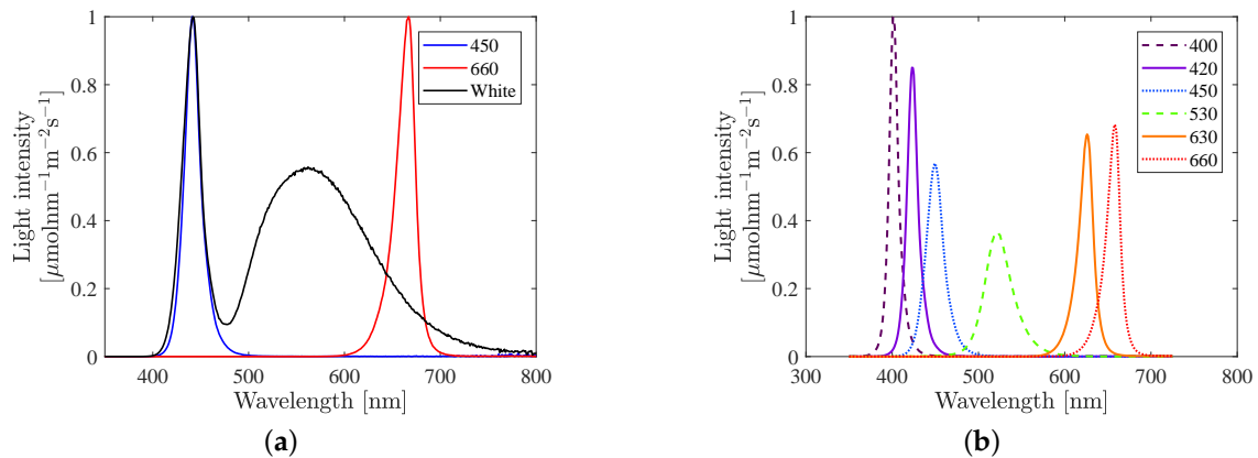
Figure 1. (a) Spectrum from the LX lamp for the blue, white and red LEDs, used to generate background light. (b) Spectrum from the RX lamp for each of the six LEDs used to generate excitation light.
