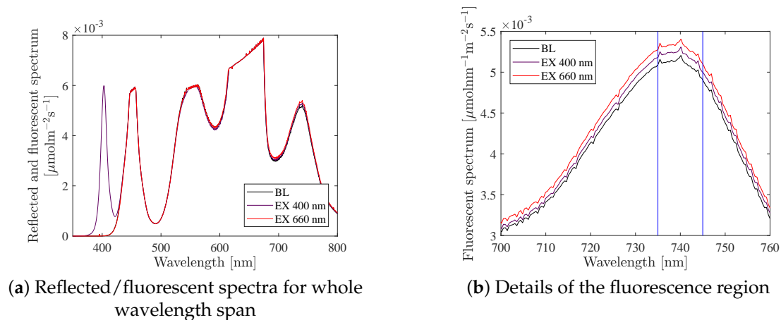
Figure 2. Reflected/fluorescent spectra for lettuce at background light intensity 500 \mu\text{mol m}^{-2} \text{s}^{-1} and spectrum with 85% red light. Three spectra are shown; for background light and with an additional excitation signal with light emitting diode (LED) 400 and LED 660 respectively. Vertical lines in plot (b), indicate the region where the spectrum is integrated to get the F740 signal according to Equation (1). Notice that the spectrometer is light saturated in wavelengths 630–670 nm, however this is outside the wavelength of interest (i.e., the span 735–745 nm).
