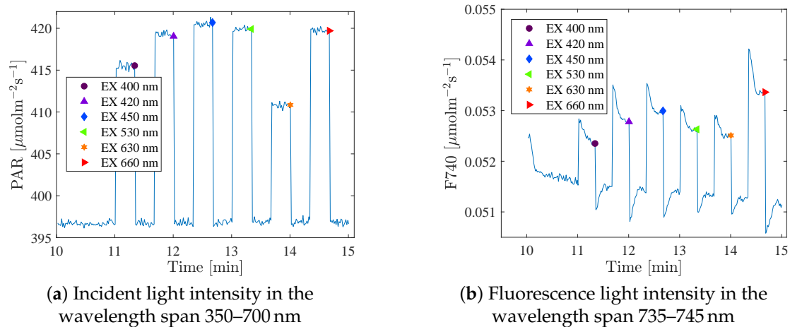
Figure A1. Measurements on lettuce, holding each intensity level at 20 s. (a) Incident and (b) fluorescence light intensity ( \mu\text{mol m}^{-2} \text{s}^{-1} ) vs. time for one background light level, i.e., background intensity 500 \mu\text{mol m}^{-2} \text{s}^{-1} and spectrum having 85% red light. An excitation step is sequentially added by each LED colour. Note that the intensity level measured during the experiment was only about 397 and not 500 \mu\text{mol m}^{-2} \text{s}^{-1} . This is because when the light level was determined, no plants were present in the experimental unit and another type of spectrometer was used.
