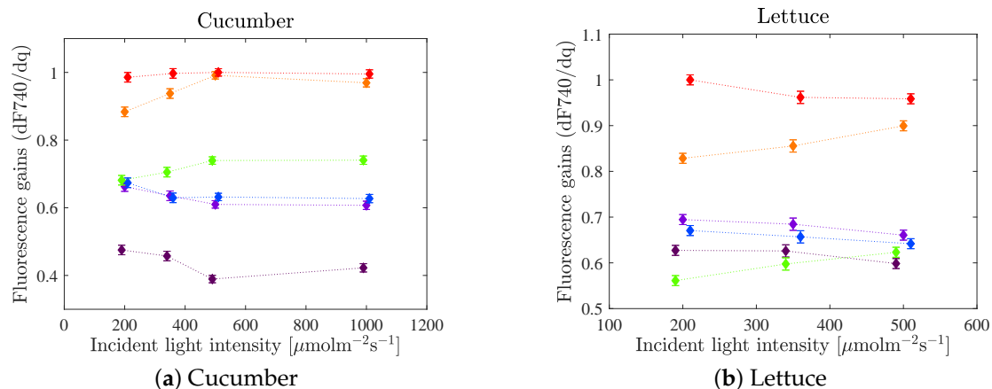
Figure 7. Mean values (and standard errors of the mean) of the fluorescence gains at each intensity level, independent of the background spectra, for (a) cucumber and (b) lettuce.
