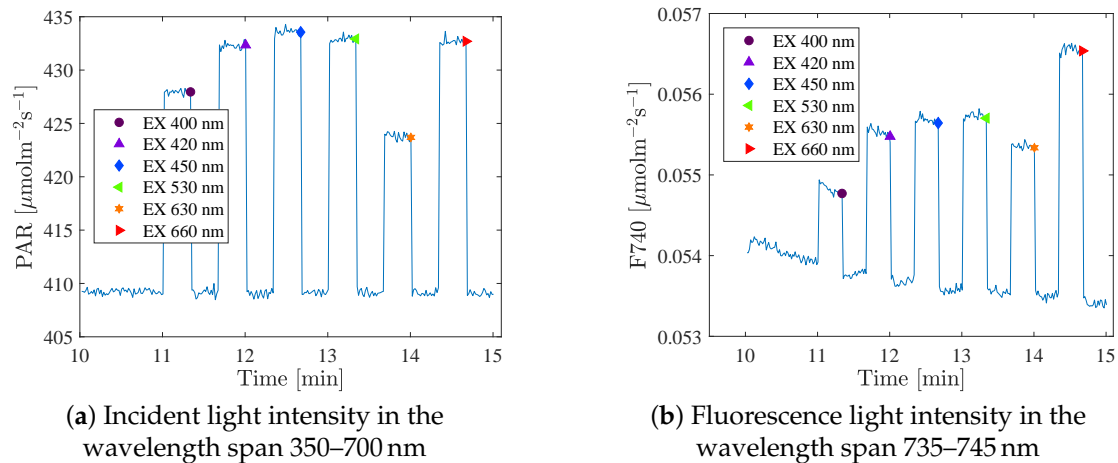
Figure A2. Measurements on cucumber, holding each intensity level at 20 s. (a) Incident and (b) fluorescence light intensity ( \mu\text{mol m}^{-2} \text{s}^{-1} ) vs. time for one background light level, i.e., background intensity 500 \mu\text{mol m}^{-2} \text{s}^{-1} and spectrum having 85% red light. An excitation step is sequentially added by each LED colour. Note that the intensity level measured during the experiment was only about 409 and not 500 \mu\text{mol m}^{-2} \text{s}^{-1} . This is because when the light level was determined, no plants were present in the experimental unit and another type of spectrometer was used.
