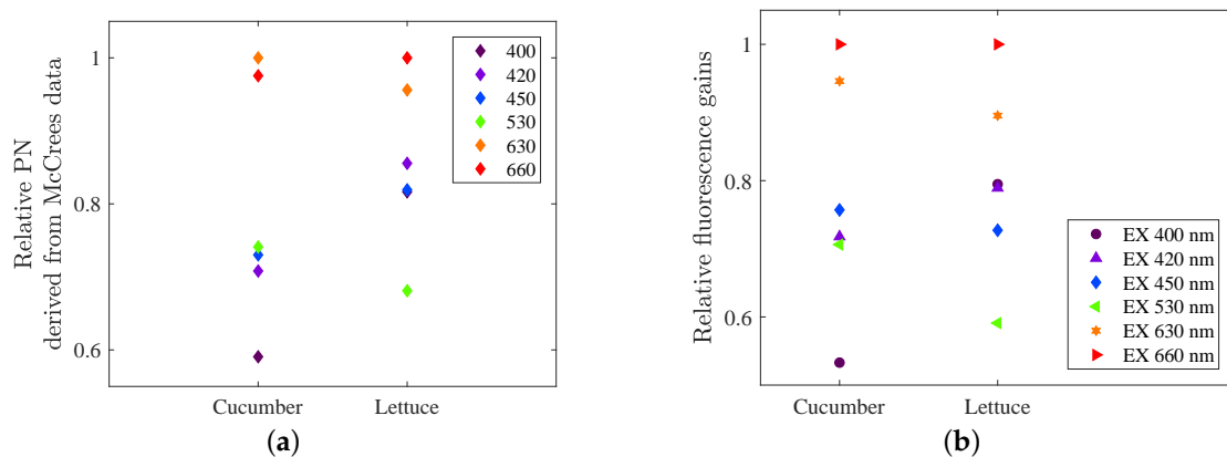
Figure 12. (a) Relative PN gain of each LED colour for cucumber and lettuce, calculated from data from McCree. (b) Experimentally derived fluorescence gains at background light intensity 160 \mu\text{mol m}^{-2} \text{s}^{-1} (set A).
