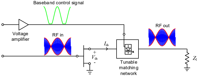
Figure 2.7: Varactor-based dynamic load modulation architecture.
