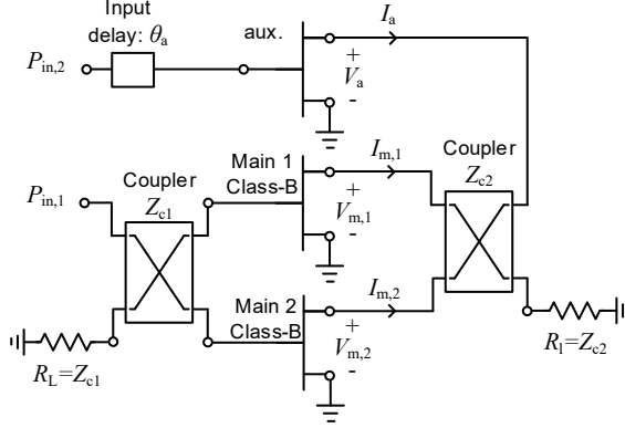
Figure 2.6: (a) Ideal load modulated balanced amplifier.
