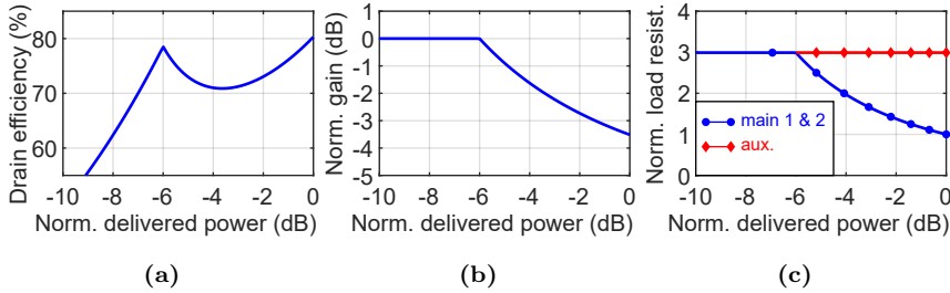
Figure 4.4: (a) Drain efficiency, (b) gain, and (c) load modulation versus normalized delivered power of the RF-input LMBA. The gain is normalized with itself at back-off. The load is normalized with R_{opt} .
