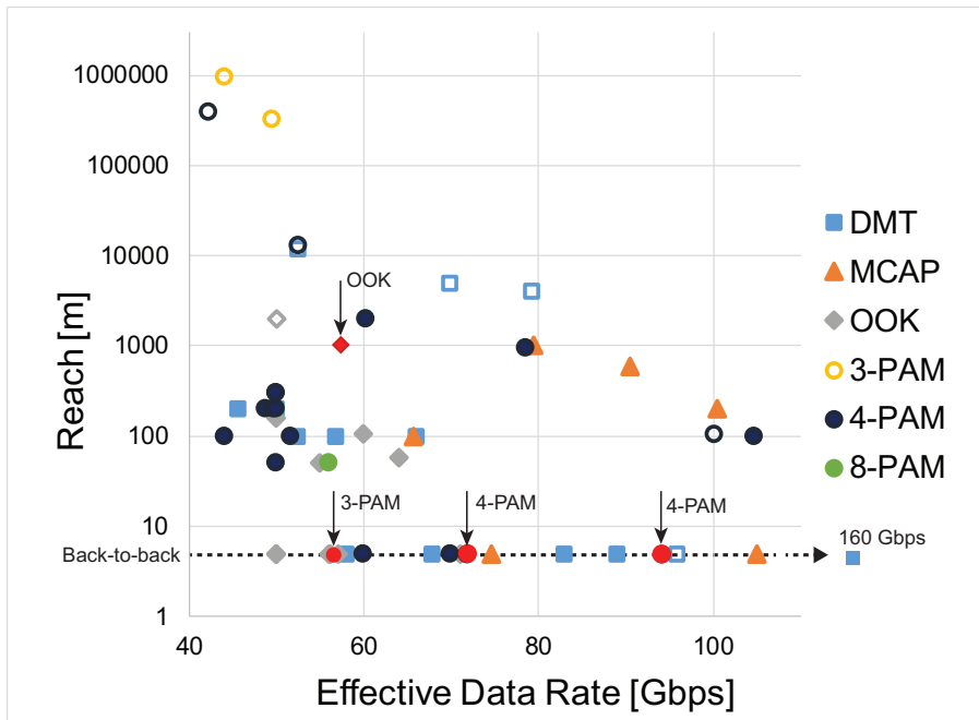
Figure 4.1: Examples of VCSEL-based links above 50 Gbps. Data rates presented are without FEC overhead. Red shapes with arrows show results in this work. Hollow markers show experiments using VCSELs and SMF with wavelengths between 1530 and 1550 nm.
