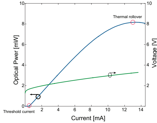
Figure 2.11: Optical output power and diode voltage versus bias current for a VCSEL.
