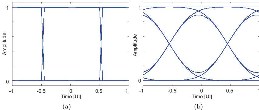
Figure 3.2: Simulated eye diagrams for OOK-NRZ with no ISI (a) and with ISI (b)
