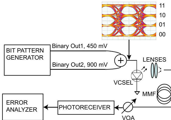
Figure 3.3: Generation of naturally labeled 4-PAM signals using a BPG and two decorrelated binary signals with the generated electrical 4-PAM signal in the inset.
