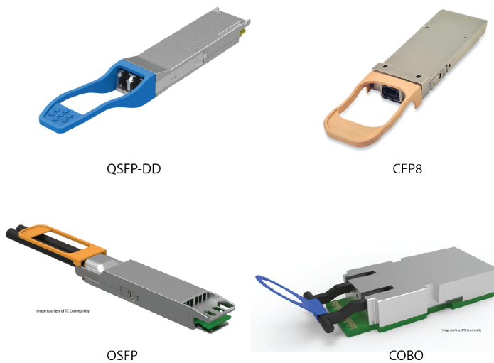
Figure 2.6: Various form factors for 400G applications in DCs: QSFP-DD, CFP8, OSFP and COBO
