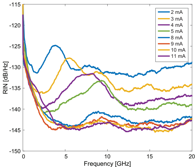
Figure 2.14: Example of RIN spectra for a multi-mode VCSEL at various bias points.
