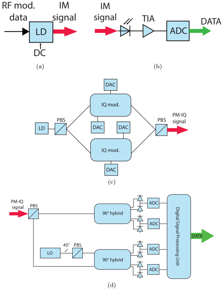
Figure 2.5: Comparison between simplified representations of IM/DD transmitter (a) and IM/DD receiver (b) and coherent, polarization multiplexed transmitter (c) and receiver (d)
