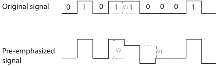
Figure 3.4: Explanatory diagram of pre-emphasis and de-emphasis using time-domain waveforms.
