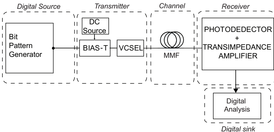
Figure 2.9: Simplified illustration of a VCSEL-based link.
