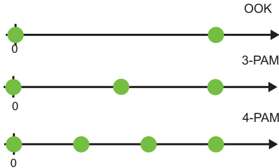
Figure 3.1: Constellation diagrams for OOK and 4-PAM
