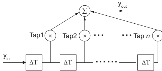
Figure 3.5: Example of how FFE pre-emphasis is generated using FIR filters.
