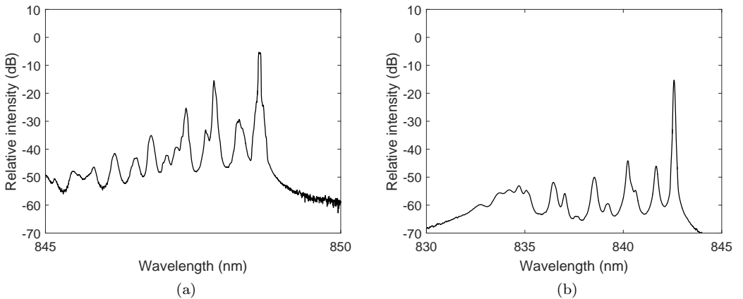
Figure 2.12: Typical output spectrum for multi-mode (a) and single-mode (b) 850 nm VCSEL at 8 mA bias and room temperature. Courtesy of Petter Westbergh.
