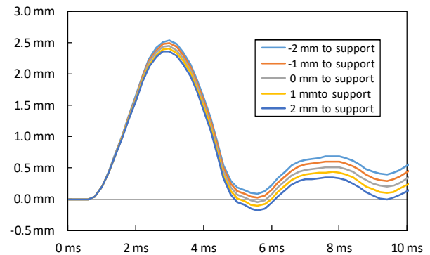
Figure 7. Vertical motion over time of Beam 12 points over support.
