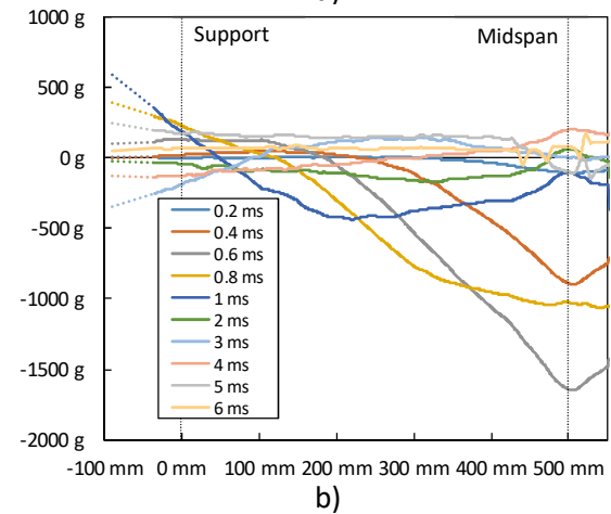
Figure 3. Measured parameters evolution for Beam 12: a) deflections; b) accelerations.
