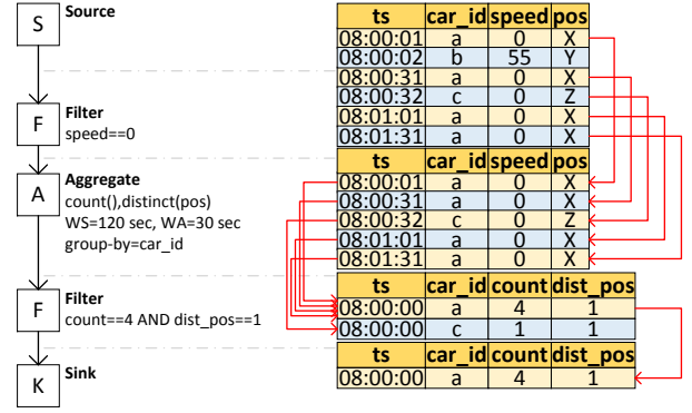
Figure 2: Sample query from Figure 1 with additional red arrows showing the contribution graph of the sink tuple.
