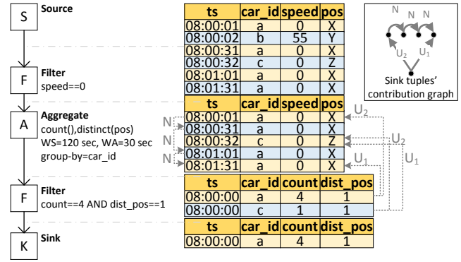
Figure 4: Sample query and execution from Figure 1 showing meta-attributes U_1 , U_2 and N as set by GeneaLog’s instrumented operators.
