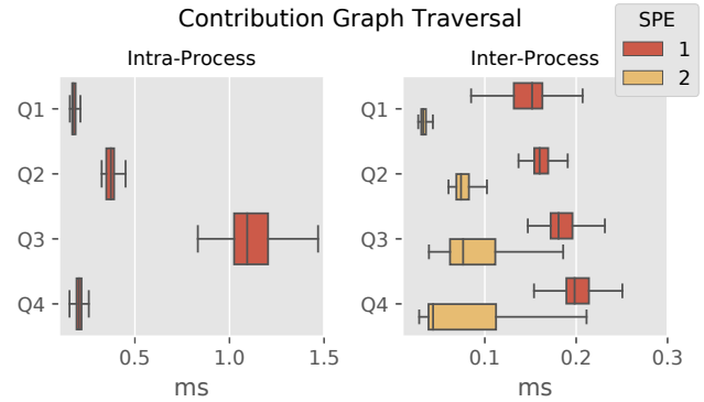
Figure 14: Time required to traverse the contribution graph for each output tuple.
