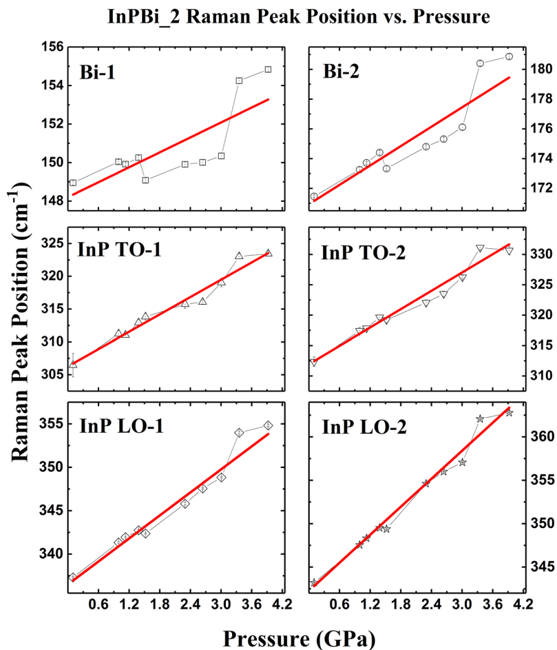
FIG. 3. Peak positions of various Raman vibration modes in InPBi measured from InPBi_2 in DAC at different hydrostatic pressures. Red lines are the linear fitting results, respectively.
