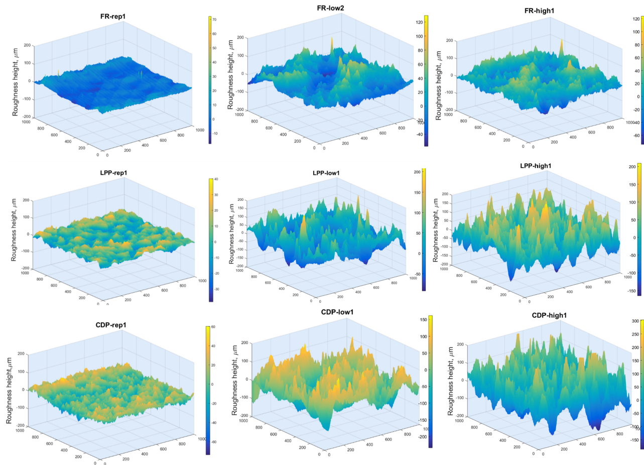
Figure 2. Topographical views of one replicate of each FR, LPP and CDP types with normal vs mimicked hull finishes. Plots from left to right represent the roughness densities. The surface texture measurement was taken at a 25 \times 25 \text{ mm}^2 area with a sampling interval of 25 \mu\text{m} using an optical surface profilometer.
