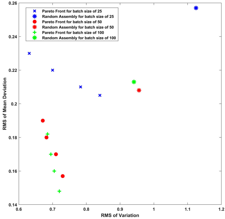
Figure 9. Pareto-Front and averages for different batch sizes of case 3.
