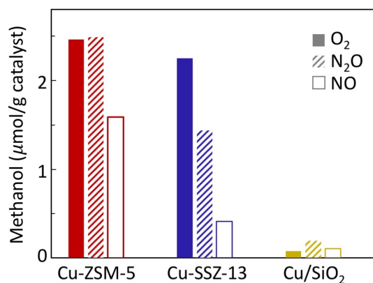
Figure 1. Methanol production over Cu-ZSM-5, Cu-SSZ-13 and Cu/SiO 2 at 1 atm using O 2 , N 2 O or NO as oxidants.
