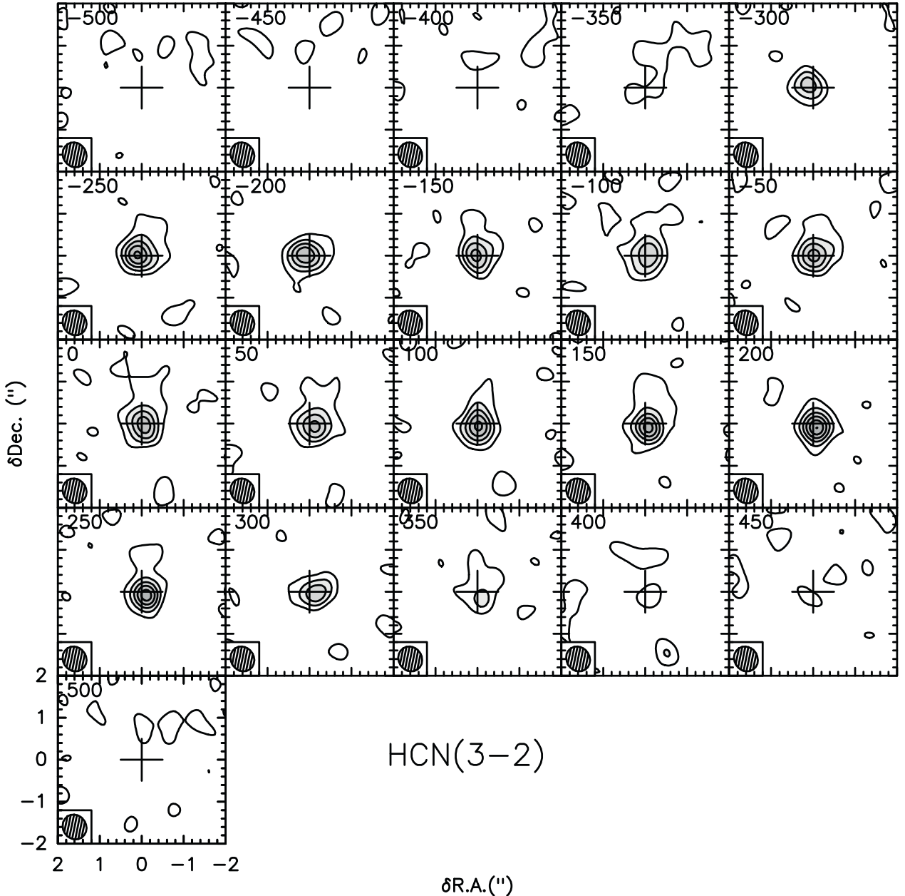
Fig. 13. Channel-velocity maps of HCN(3–2) in the velocity range [-500, 500] \text{km s}^{-1} with steps of 50 \text{ km s}^{-1} . Contours go from 6.5 \text{ mJy beam}^{-1} ( 5\sigma ) to 56 \text{ mJy beam}^{-1} with a spacing of 10 \text{ mJy beam}^{-1} . We highlight the significantly smaller spatial scale relative to the channel map of the (1–0) line shown in Fig. 11. The synthesised beam is plotted in the bottom-left corner. North is up and east is to the left.
