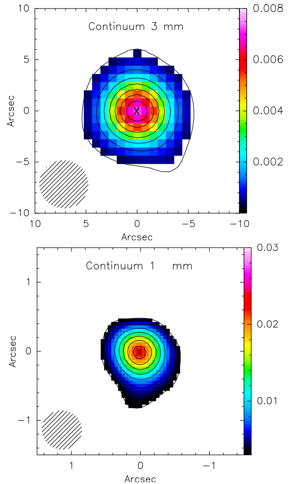
Fig. 1. Continuum maps at 3\text{ mm} and 1\text{ mm} . Contour levels start at a significance of 5\sigma with respect to the rms measured in both images (rms = 0.07\text{ mJy channel}^{-1} and 0.6\text{ mJy channel}^{-1} for the 3\text{ mm} and 1\text{ mm} maps respectively). The contour steps are 1 and 3\text{ mJy km s}^{-1}\text{ beam}^{-1} . The crosses at the centres mark the continuum peaks, which we take as the location of the northern nuclear source (see Sect. 1). The synthesised beams are shown in the bottom-left corner. The colour flux scales are in \text{Jy km s}^{-1}\text{ beam}^{-1} .
