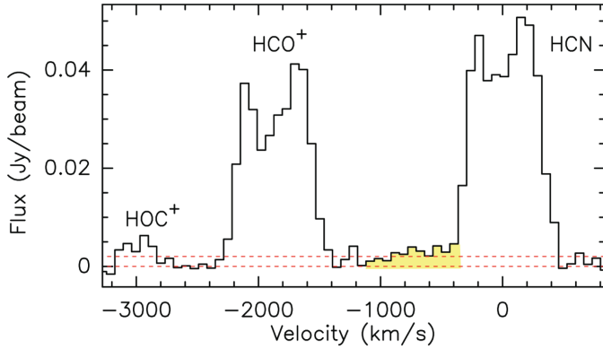
Fig. 5. Spectrum of the central pixel for the (J - J') = (3 - 2) lines of HCN, \text{HCO}^+ and \text{HOC}^+ . The baseline of order 0 and the 3 \times \text{rms} flux (calculated at the final velocity resolution of 68 \text{ km s}^{-1} ) are marked with horizontal dashed lines. The outflow emission at the blue-shifted velocities of HCN is highlighted in yellow.
