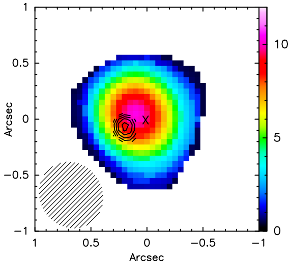
Fig. 17. \text{HCO}^+(3-2) blue-shifted intensity colours (in units of \text{Jy km s}^{-1} \text{beam}^{-1} ) integrated from -300 \text{ km s}^{-1} to 0 \text{ km s}^{-1} with \text{HCO}^+(3-2) contours (starting from 3\sigma = 3.3 \text{ mJy beam}^{-1} ) over-plotted with steps of 10 \text{ mJy beam}^{-1} . The cross at the centre marks the continuum peak. The synthesised beam is shown in the bottom-left corner.
