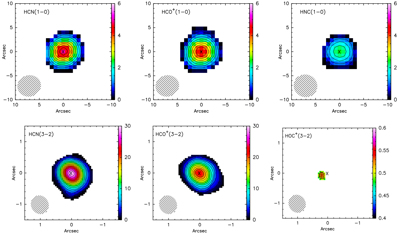
Fig. 6. Integrated intensities (moment zero maps). Contour levels for HCN, HCO + and HNC (1–0) go from 0 to 6 Jy km s −1 beam −1 with a step of 0.5 Jy km s −1 beam −1 . For HCN (3–2) and HCO + (3–2) the levels range from 2 to 30 Jy km s −1 beam −1 with a step of 2 Jy km s −1 beam −1 . For HOC + (3–2), the contours are from 0.4 to 0.6 Jy km s −1 beam −1 with a step of 0.04 Jy km s −1 beam −1 . We highlight the different scales between the (1–0) and the (3–2) lines. The crosses in the centre of each panel indicate the location of the nuclear source. The synthesised beam is shown in the bottom-left corner of each panel. North is up, and east is to the left.
