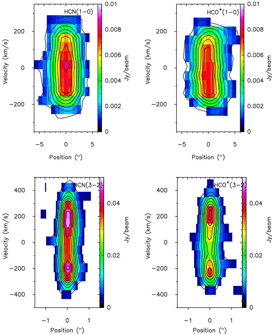
Fig. 9. Position-velocity (p-v) maps of HCN and HCO + . The cuts along the axes of rotation are shown by the dashed lines in Fig. 8. Contour steps of the (1–0) maps go from 0.9 mJy beam -1 (3 \sigma ) to 7.9 mJy beam -1 with steps of 1 mJy beam -1 . For the (3–2) maps, contours go from 3.9 mJy beam -1 (3 \sigma ) to 59 mJy beam -1 with steps of 5 mJy beam -1 .
