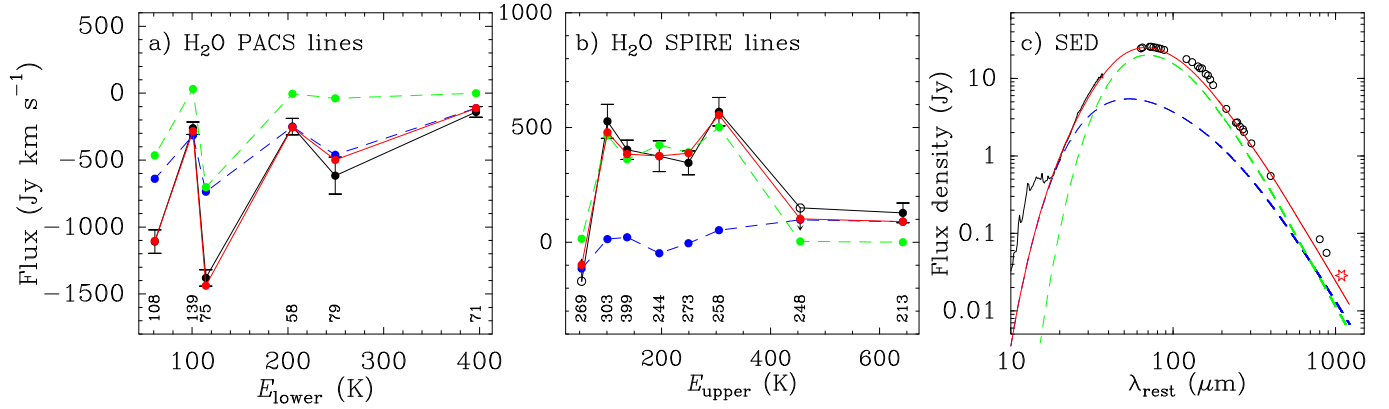
Fig. 15. Comparison between the observed (black symbols) and modelled (coloured symbols and lines) H 2 O fluxes in Mrk 273 within panel a : PACS and panel b : SPIRE. The model includes two components: the core (in blue), which accounts for most absorption lines observed within PACS, and the inner disc (in green), which dominates the emission of the sub-mm lines with E_{\text{upper}} < 400 K observed with SPIRE (see Table 4). Red colours and symbols indicate total modelled fluxes. The numbers at the bottom of panels a and b indicate rounded-up transition wavelengths in \mu\text{m} . Panel c : the SED of Mrk 273, including the Spitzer / IRS spectrum, Herschel /PACS and SPIRE continuum data from observations of both H 2 O and OH lines, sub-mm data at 800 and 880 \mu\text{m} (Rigopoulou et al. 1996; Wilson et al. 2008), and our measured flux density at 1 mm (starred-red symbol), is compared with the prediction of our composite model.
