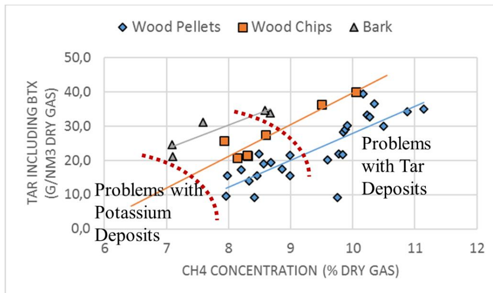
Figure 3.5: Concentration of tar in dry part of the Raw Gas as a function of CH 4 concentration, from [19].
