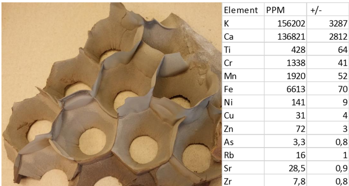
Figure 3.6: Picture of ash deposits extracted from the top of the product gas cooler and the results of the XRF analysis of the deposits, from [19].
