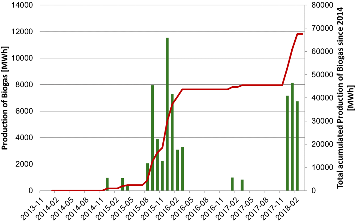
Figure 3.2: Biogas production, each bar represents a continuous run and the line is the accumulated production.
