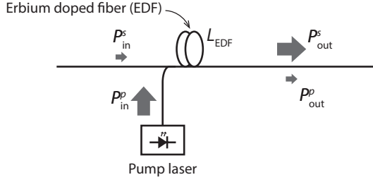
Figure 3.1: Schematic of a basic EDFA, with one co-propagating pump.
